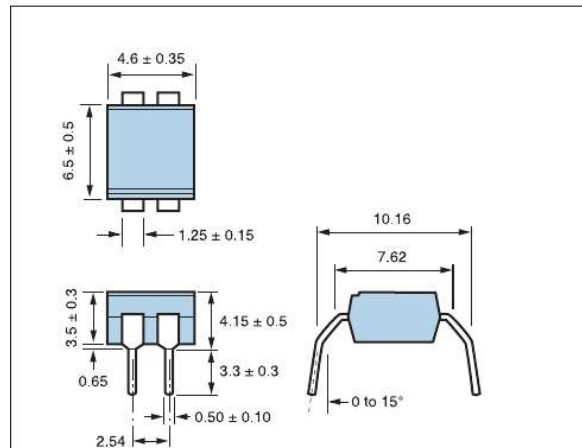
L1 — DIP4 Thru-Hole Gull Wing
