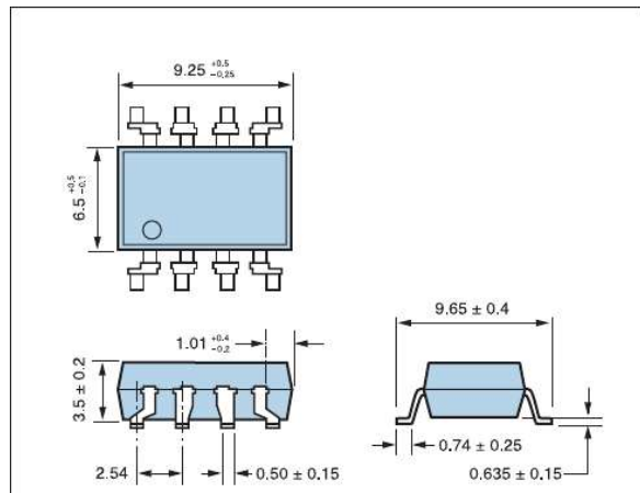
L3 — SMT DIP8 Gull Wing
