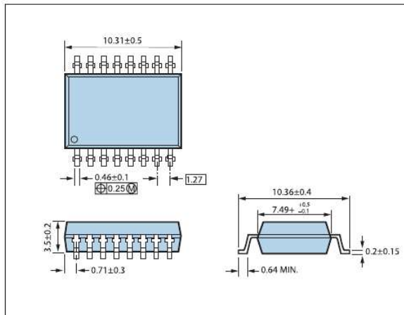
16-Pin SSOP
