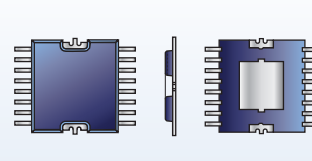
GR Package
