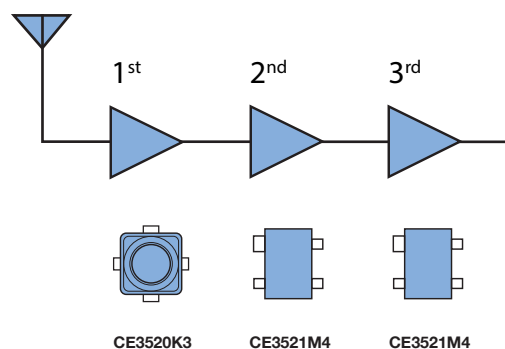
20GHz LNB
