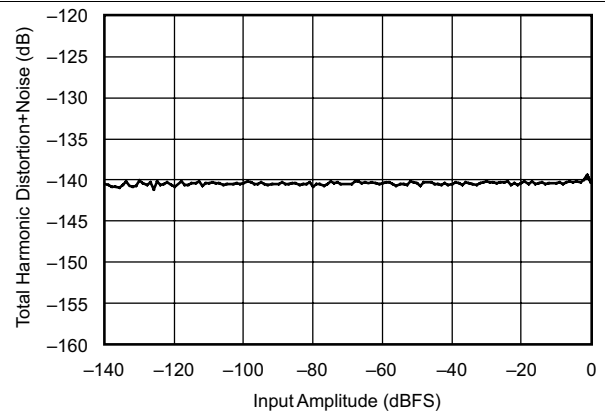
Figure 40. THD+N vs Input Amplitude f_{IN} = 1\text{ kHz}
