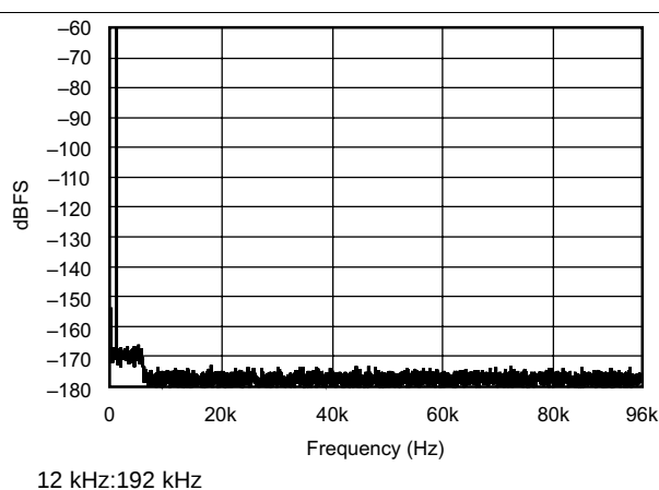
Figure 2. FFT With 1-kHz Input Tone at -60 dBFS
