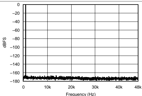
Figure 11. FFT With 1-kHz Input Tone at 0 dBFS
