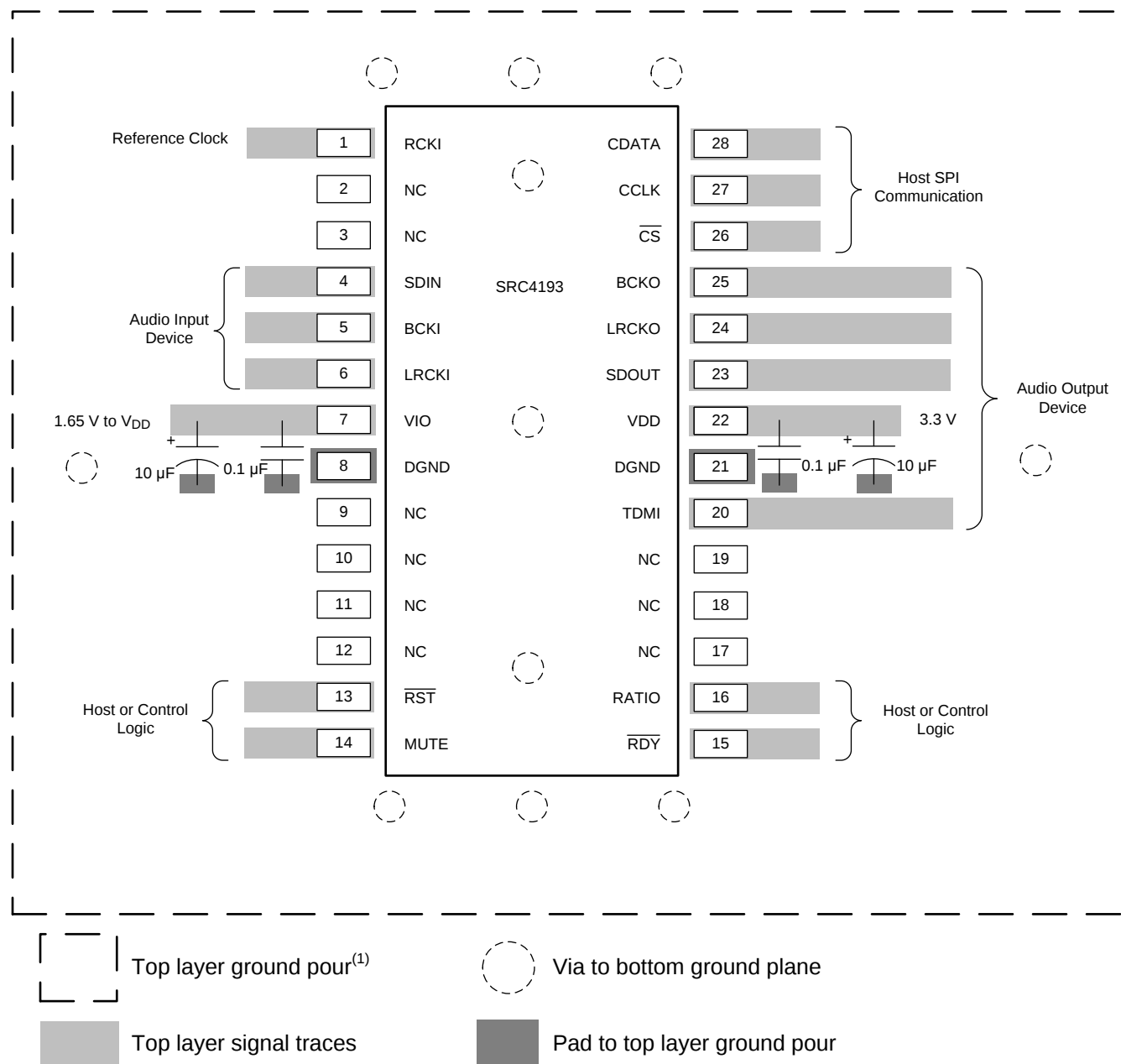
Figure 82. SRC4193 Layout Example
