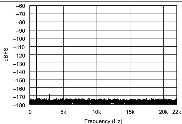
Figure 28. FFT With 1-kHz Input Tone at -60 dBFS
