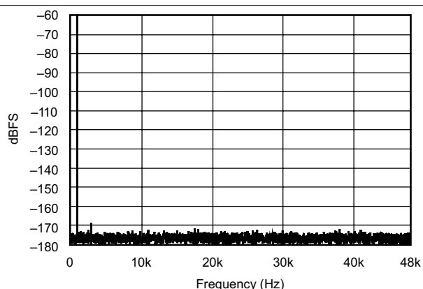
Figure 30. FFT With 1-kHz Input Tone at -60 dBFS
