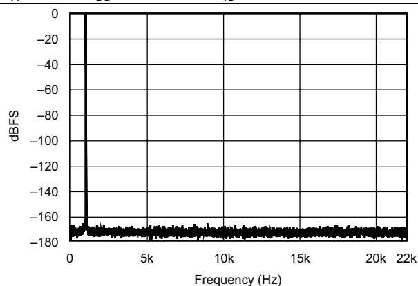
Figure 27. FFT With 1-kHz Input Tone at 0 dBFS
