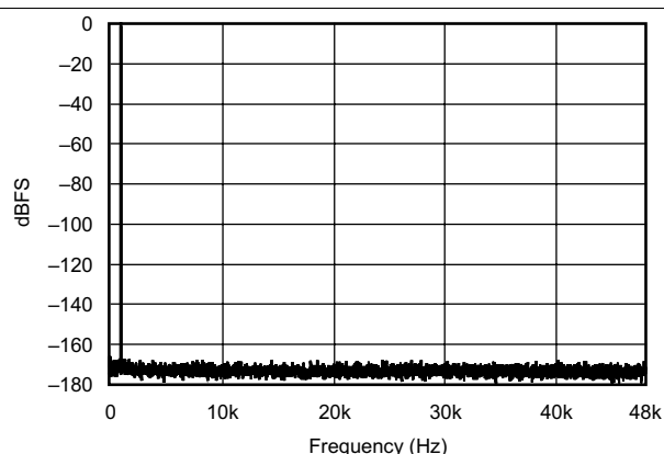
Figure 29. FFT With 1-kHz Input Tone at 0 dBFS
