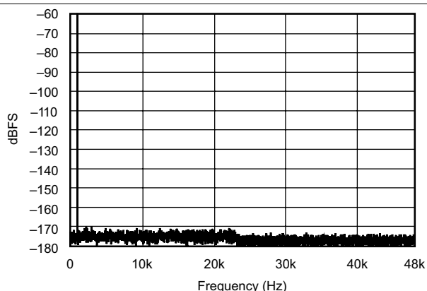
Figure 12. FFT With 1-kHz Input Tone at -60 dBFS
