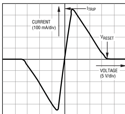
Typical V-I Characteristics (TBU-CX050-VTC-WH with R_{\text{ext}} = 1 \Omega )
