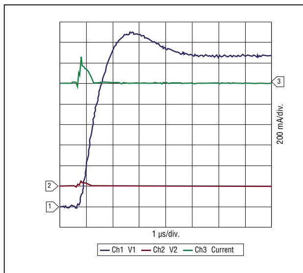
P850-G Power Fault, 230 Vrms, 25 A
