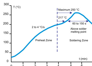
Fig. 3. Reflow Temperature Profile for Pb-free Soldering
