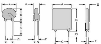
Fig.3 Lead Size : 20AWG Ø0.81 mm Diameter
