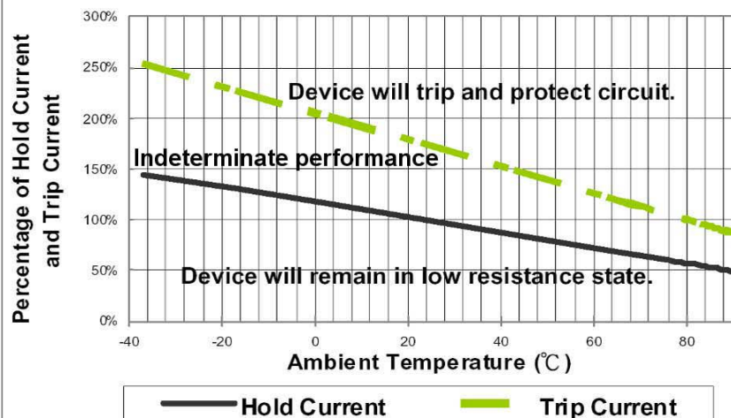
Hold &amp; Trip Current and Thermal Derating Curve
