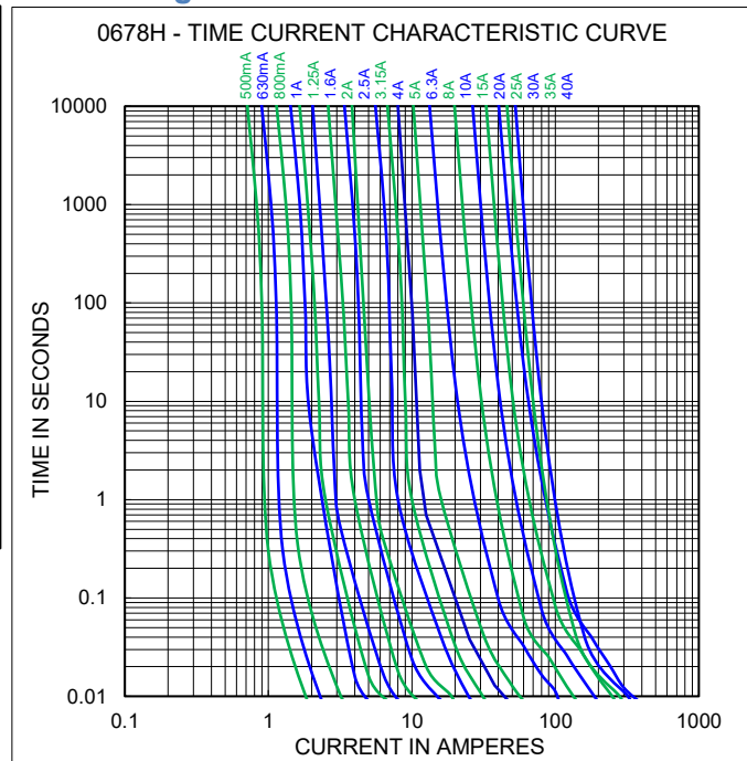
Average Time Current Curve
