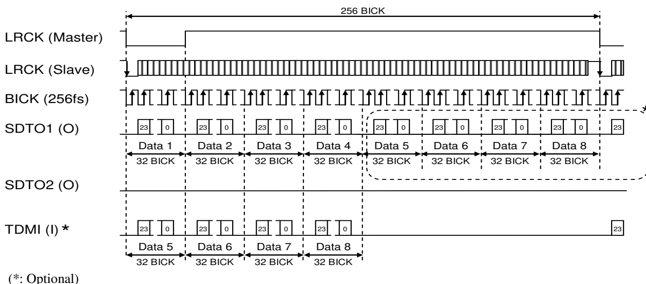
Figure 17. Model Timing (TDM256 Mode (I 2 S))
