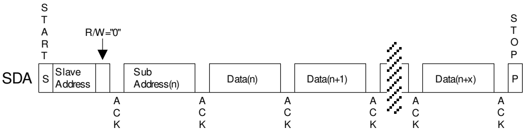
Figure 33. Data Transfer Sequence at The I²C-Bus Mode
