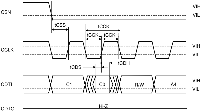
Figure 10. WRITE/READ command input timing (4-wire serial mode)
