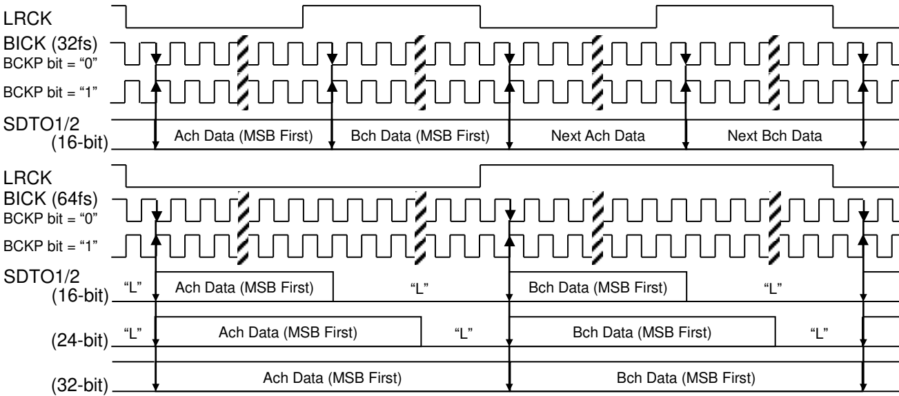
Figure 18. Mode 0/4 Timing (Normal mode, I²S Compatible)
