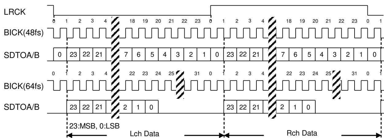
Figure 25. Mode 3 Timing (Stereo Mode, 24bit I 2 S compatible)
