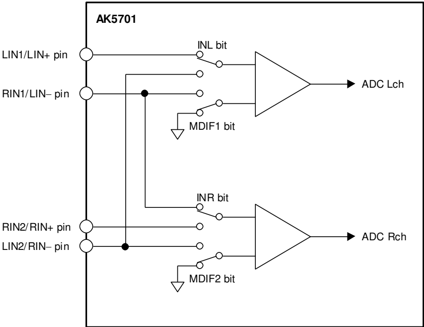
Figure 36. Mic/Line Input Selector
