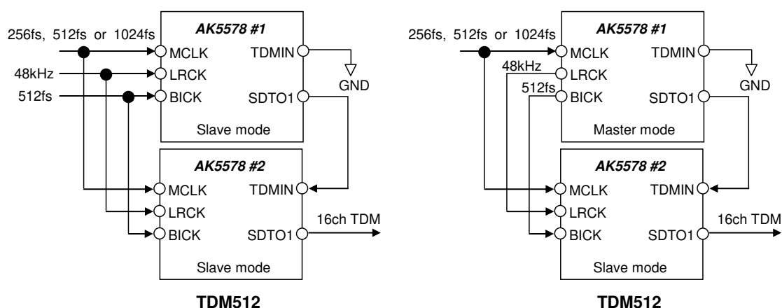
Figure 29. Cascade Connection
