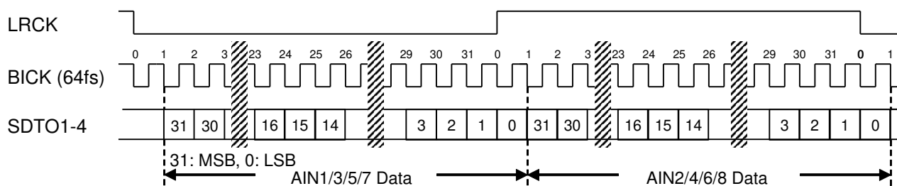
Figure 33. Mode 3/7 Timing (Normal Output, Normal/Double/Quad Speed Mode, I²S Compatible, 32-bit)
