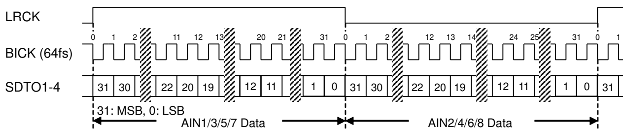
Figure 32. Mode 2/6 Timing (Normal Output, Normal/Double/Quad Speed Mode, MSB Justified, 32-bit)
