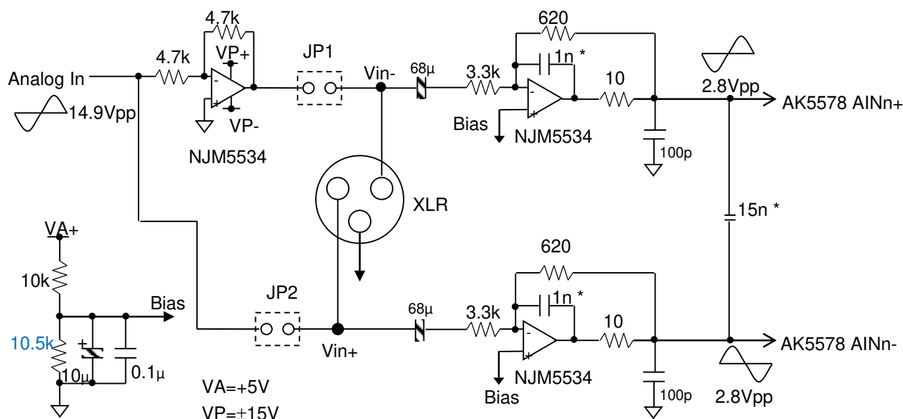
Figure 76. Input Buffer Example
