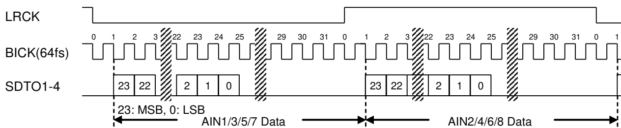
Figure 31. Mode 1/5 Timing (Normal Output, Normal/Double/Quad Speed Mode, I 2 S Compatible, 24-bit)
