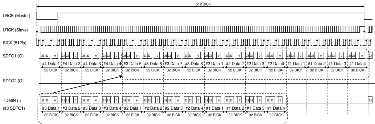
Figure 51. Mode 41/45 Timing (TDM512 mode, I²S Compatible, 24-bit)
