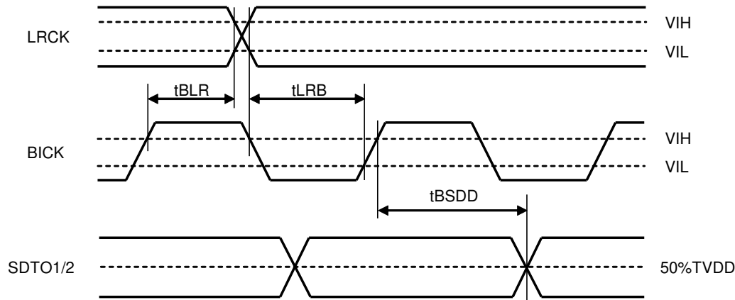
Figure 20. Audio Interface Timing (Normal & Slave mode: fs=384kHz, 768kHz)
