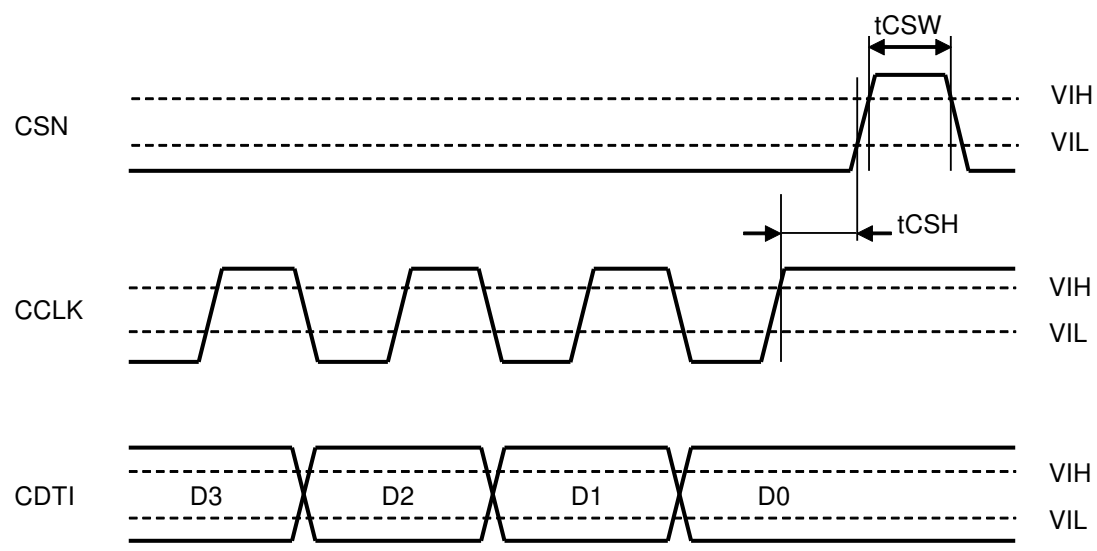
Figure 26. WRITE Data Input Timing (3-wire Serial mode)
