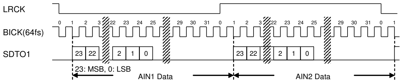
Figure 31. Mode 1/5 Timing (Normal mode, Normal/Double/Quad Speed mode, I²S Compatible, 24-bit)
