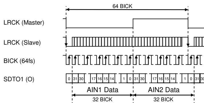
Figure 41. Mode 15/23 Timing (Normal mode, OCT/HEX Speed mode, I²S Compatible, 32-bit)
