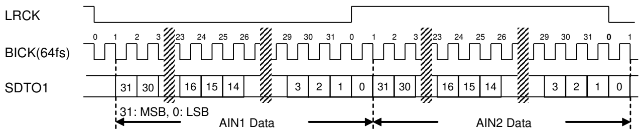
Figure 33. Mode 3/7 Timing (Normal mode, Normal/Double/Quad Speed mode, I²S Compatible, 32-bit)
