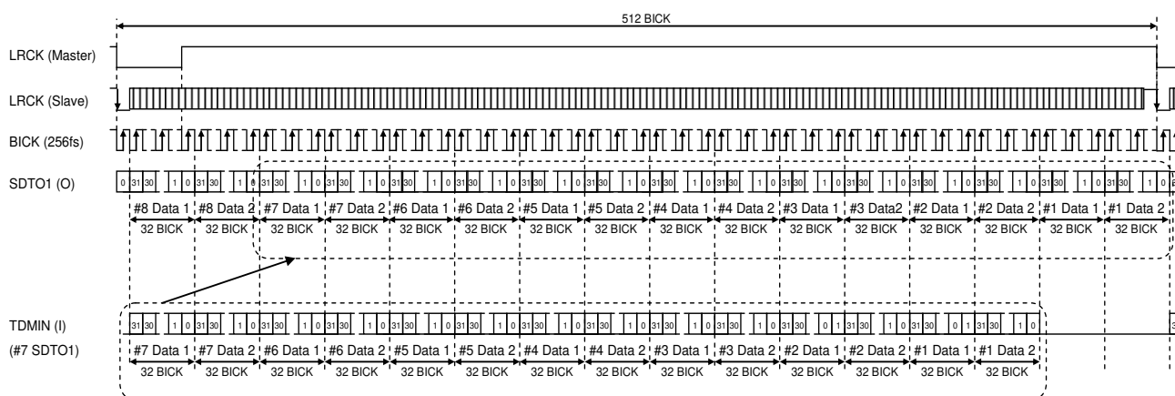
Figure 53. Mode 43/47 Timing (TDM512 mode, I²S Compatible, 32-bit)
