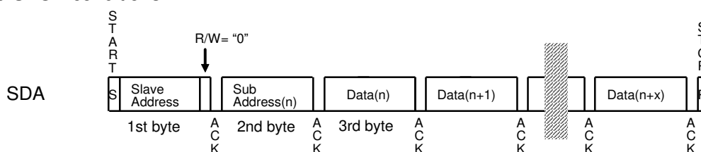
Figure 66. Data Transfer Sequence at the I 2 C-Bus Mode
