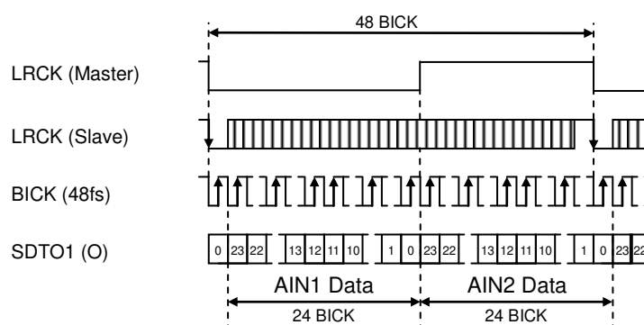
Figure 37. Mode 11/19 Timing (Normal mode, OCT/HEX Speed mode, I²S Compatible, 24-bit)
