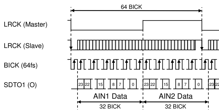
Figure 39. Mode 13/21 Timing (Normal mode, OCT/HEX Speed mode, I²S Compatible, 24-bit)
