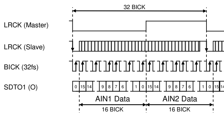
Figure 35. Mode 9/17 Timing (Normal mode, OCT/HEX Speed mode, I²S Compatible, 16-bit)
