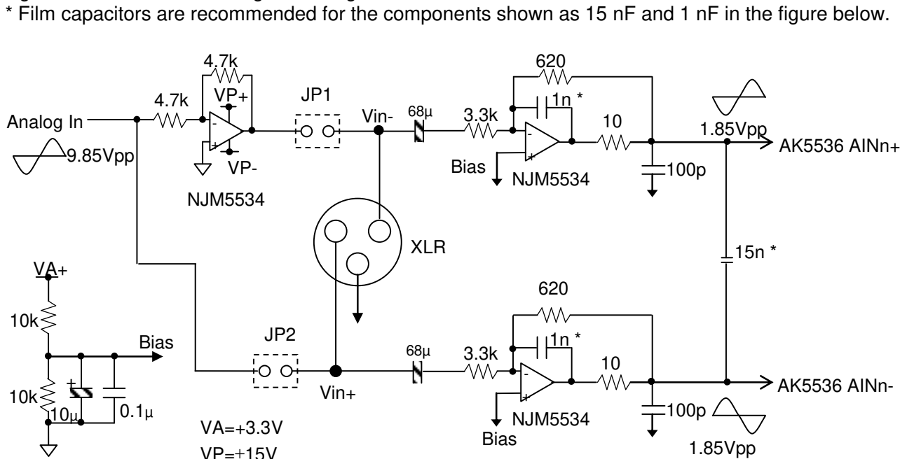
Figure 73. Input Buffer Example1
