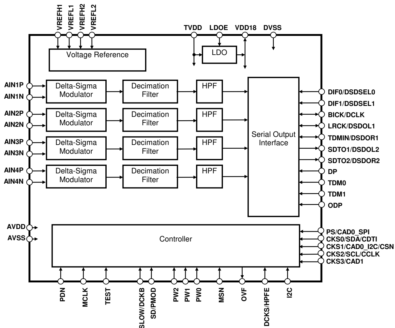
Figure 1. Block Diagram
