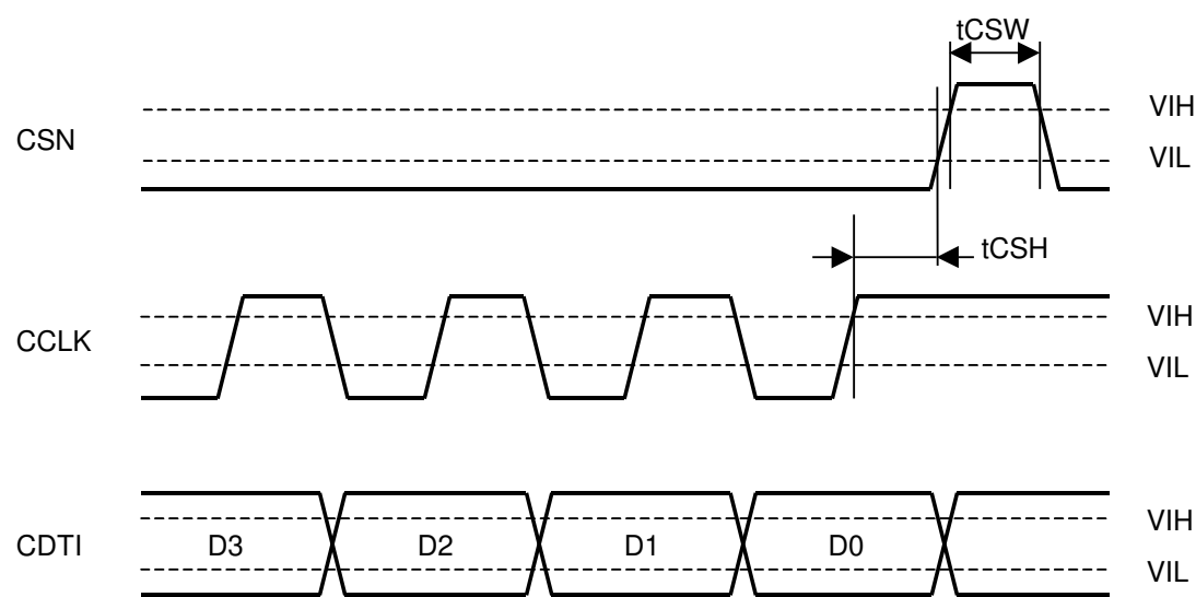
Figure 26. WRITE Data Input Timing (3-wire Serial mode)
