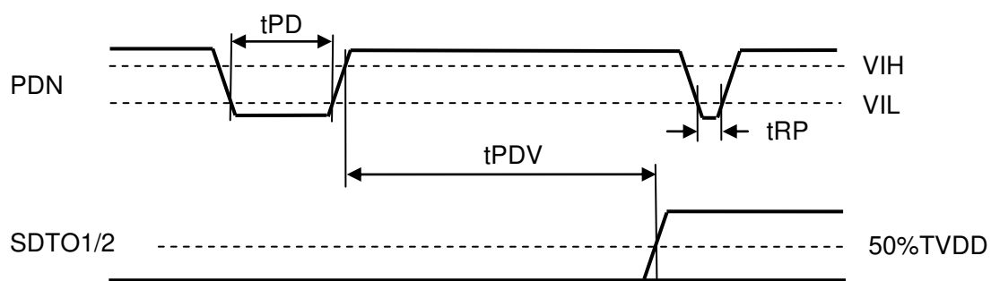
Figure 28. Power-down &amp; Reset Timing
