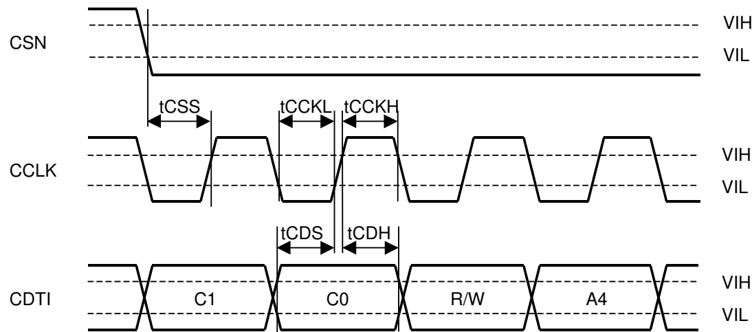
Figure 25. WRITE Command Input Timing (3-wire Serial mode)
