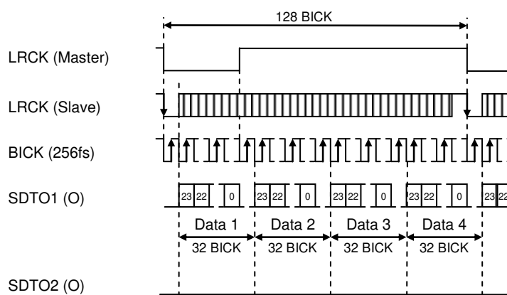
Figure 43. Mode 25/29 Timing (TDM128 mode, I 2 S Compatible)
