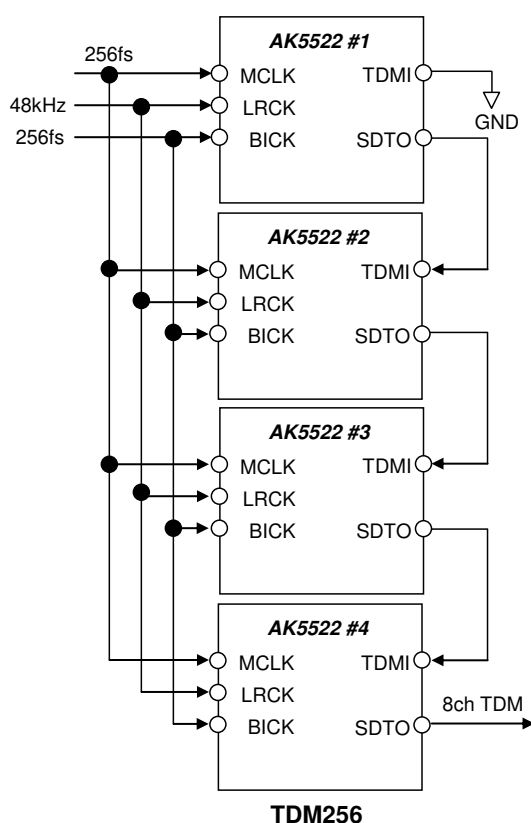
Figure 39. Cascade Connection
