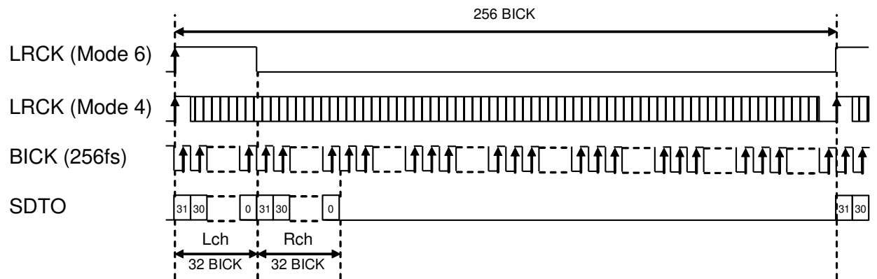
Figure 25. Mode 4/6 Timing (TDM256 mode, MSB justified)
