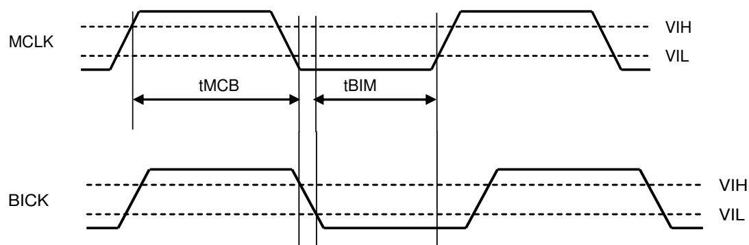
Figure 34. Audio Interface Timing (Slave mode, TDM Mode \text{MCLK}=\text{BICK} )
