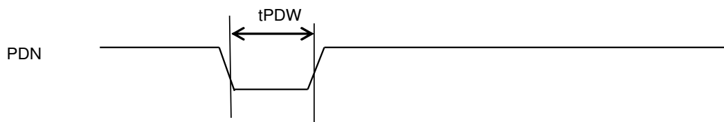
Figure 20. Reset &amp; Calibration Timing
