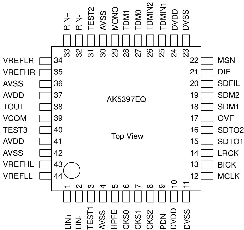
Figure 2. Pin Configurations
