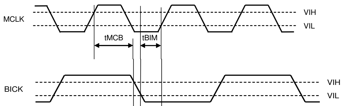
Figure 33. Audio Interface Timing (Slave mode, TDM Mode \text{MCLK}=2 \times \text{BICK} )
