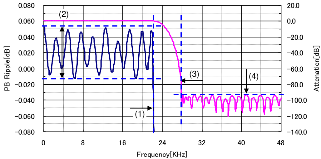
Figure 8 Short Delay Filter Normal Mode
