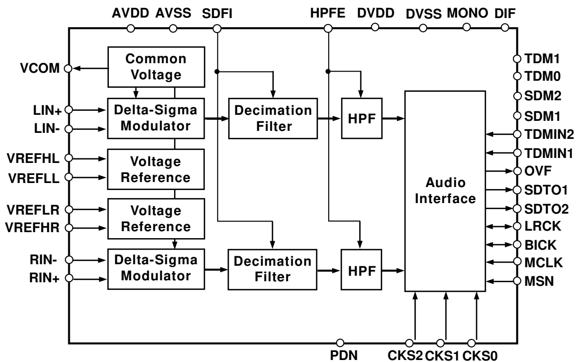
Figure 1. Block Diagram
