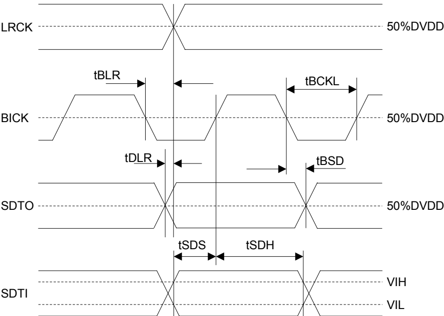
Figure 10. Audio Interface Timing
