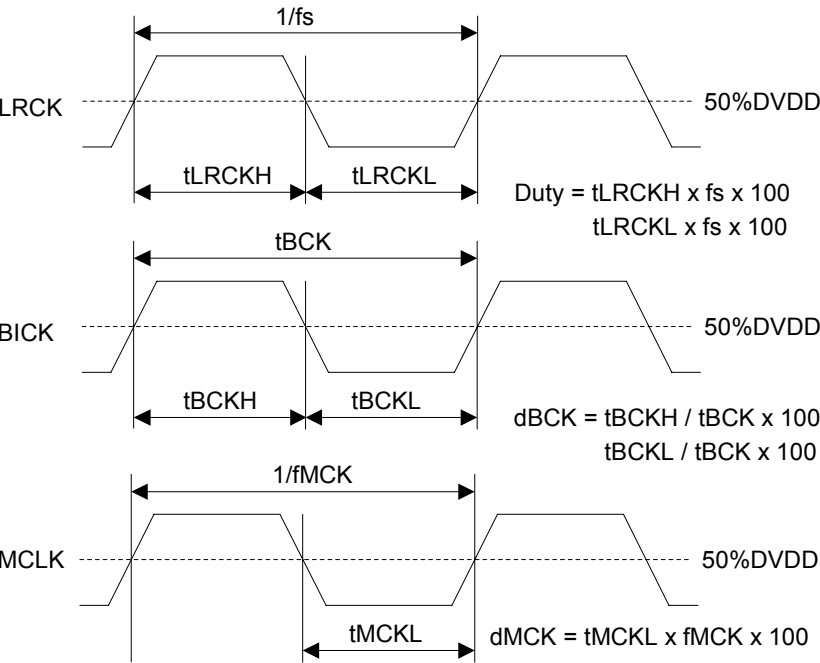
Figure 9. Audio Clock Timing
