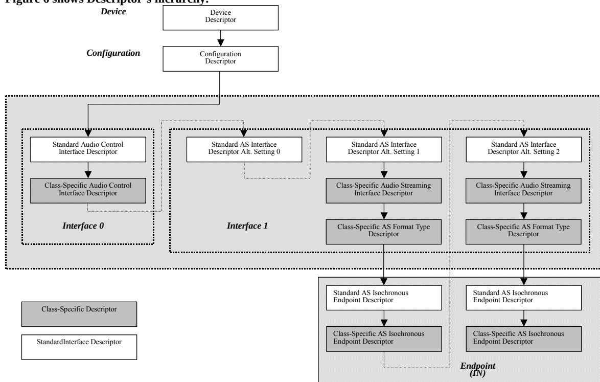
Figure 6. Descriptor Hierarchy
