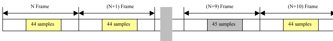
Figure 7. Synchronization
