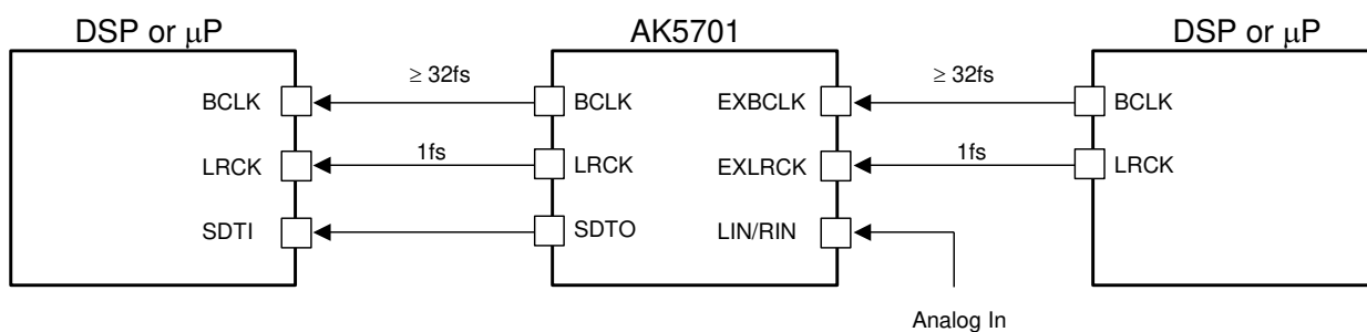
Figure 25. Slave & Bypass Mode
