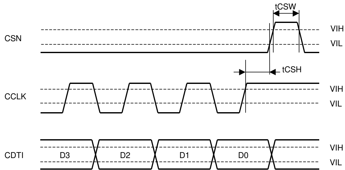
3 Wire Serial Mode WRITE Data Input Timing
