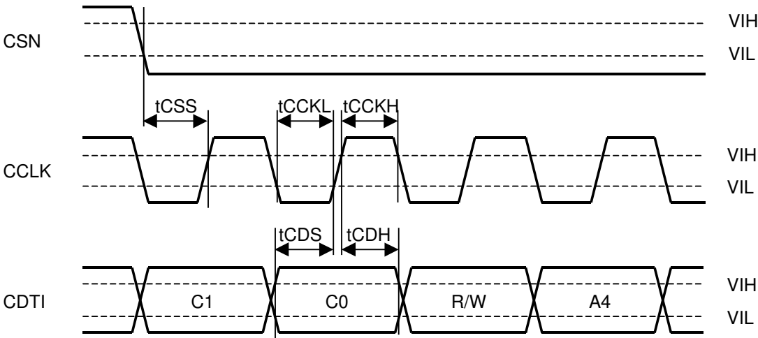
3 Wire Serial Mode WRITE Command Input Timing
