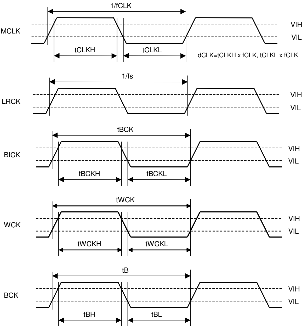
Clock Timing
