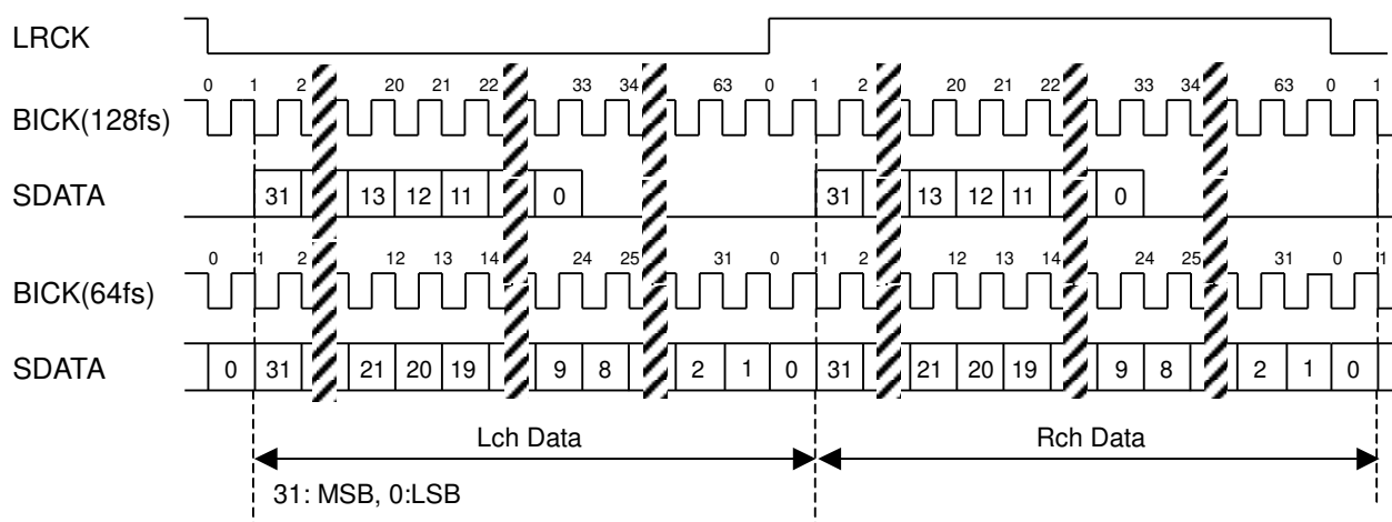
Figure 17. Mode 7 Timing
