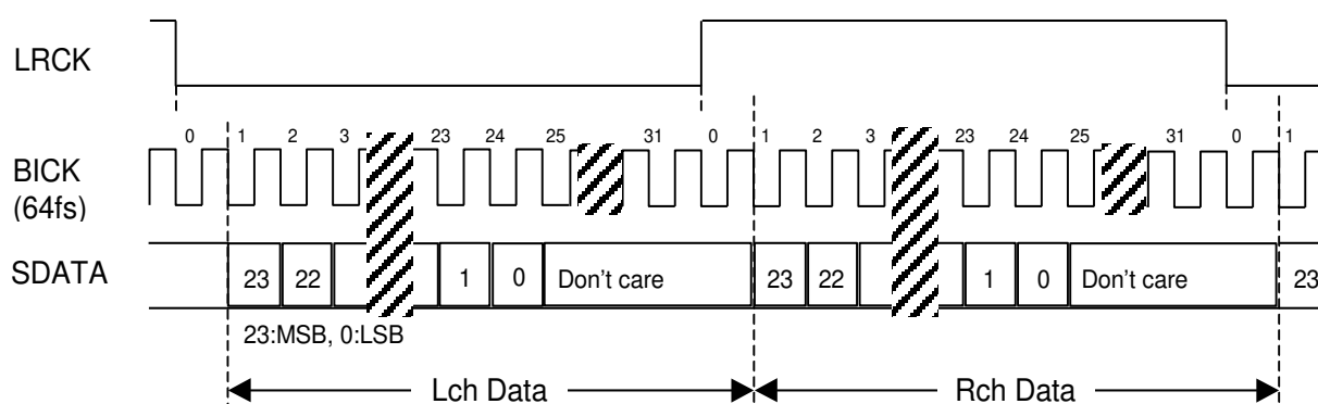
Figure 14. Mode 3 Timing
