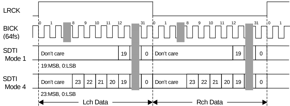
Figure 2. Mode 1, 4 Timing
