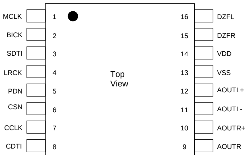
PIN/Function
