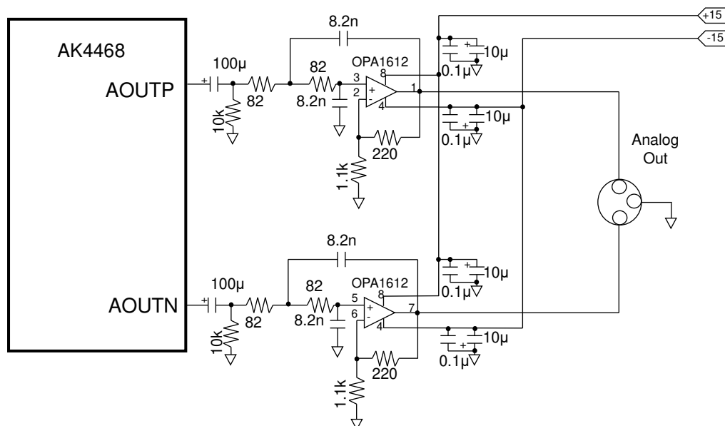
Figure 78. External LPF Circuit Example 3 ( f_c = 174 \text{ kHz} (Typ), Q = 0.5 (Typ))
