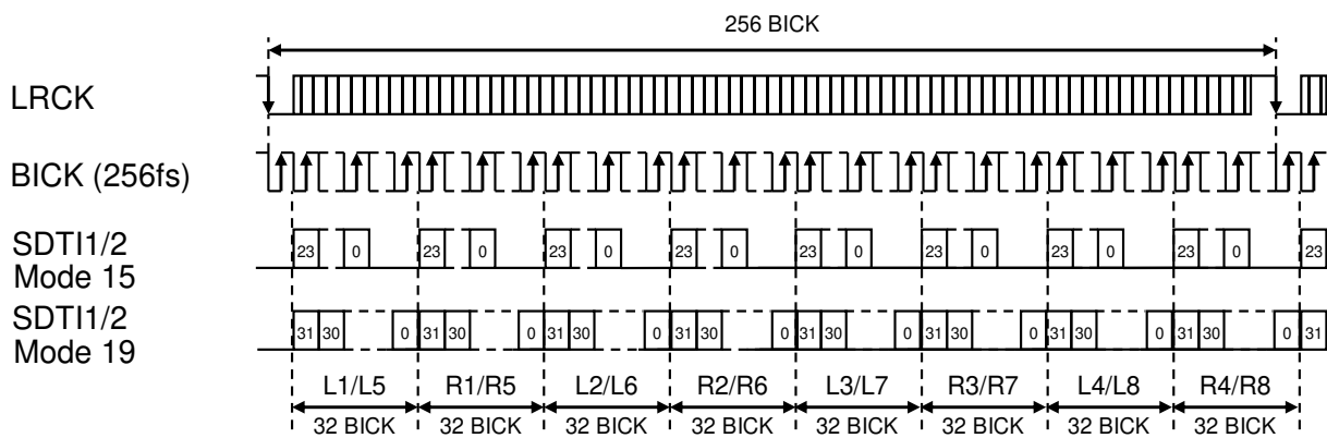
Figure 33. Mode 15/19 Timing
