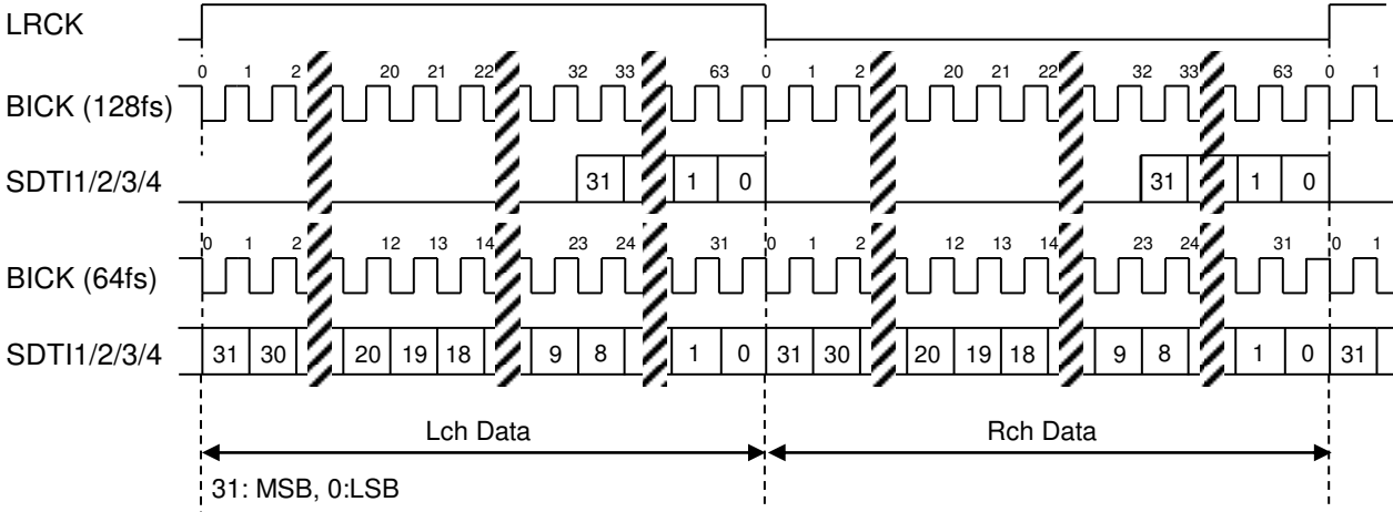
Figure 26. Mode 5 Timing
