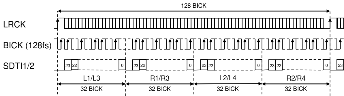
Figure 31. Mode 10 Timing
