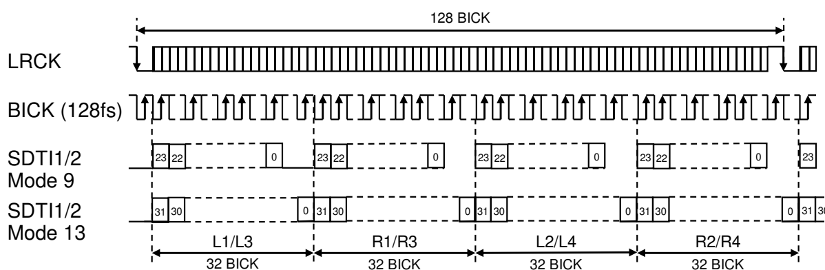
Figure 30. Mode 9/13 Timing
