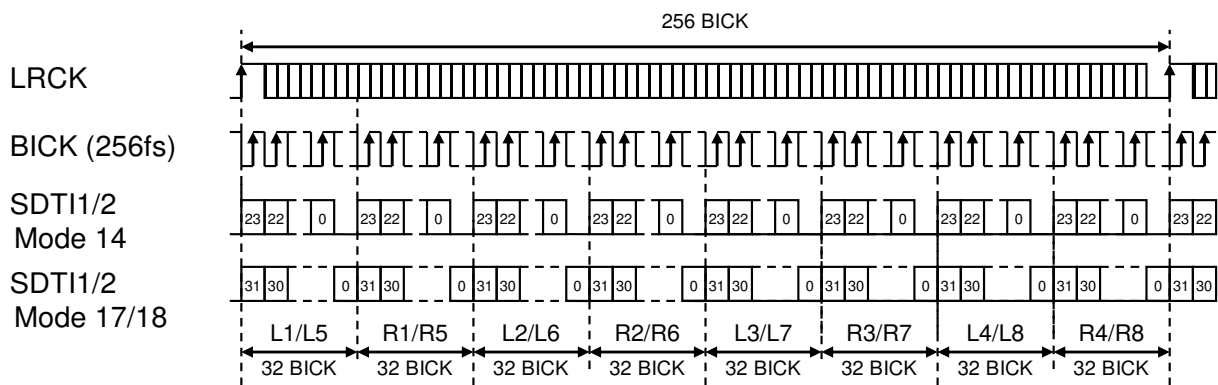
Figure 32. Mode 14/17/18 Timing
