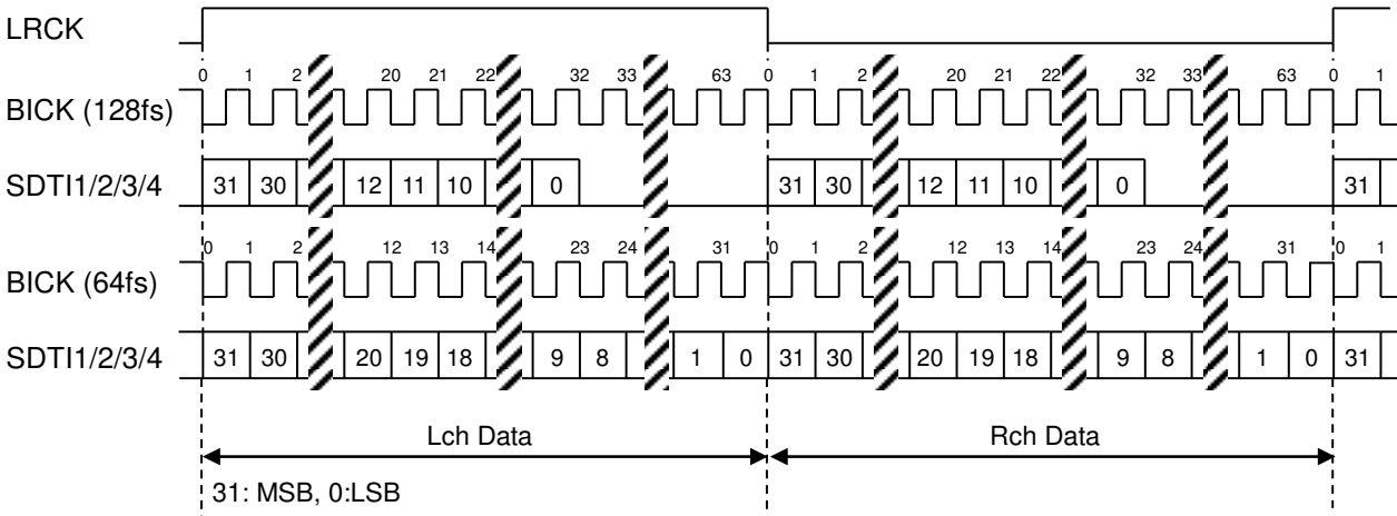
Figure 27. Mode 6 Timing
