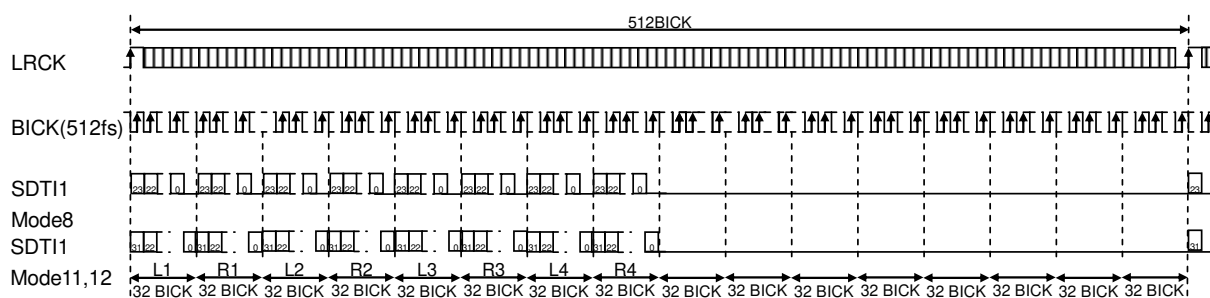
Figure 30. Mode 20/23/24 Timing
