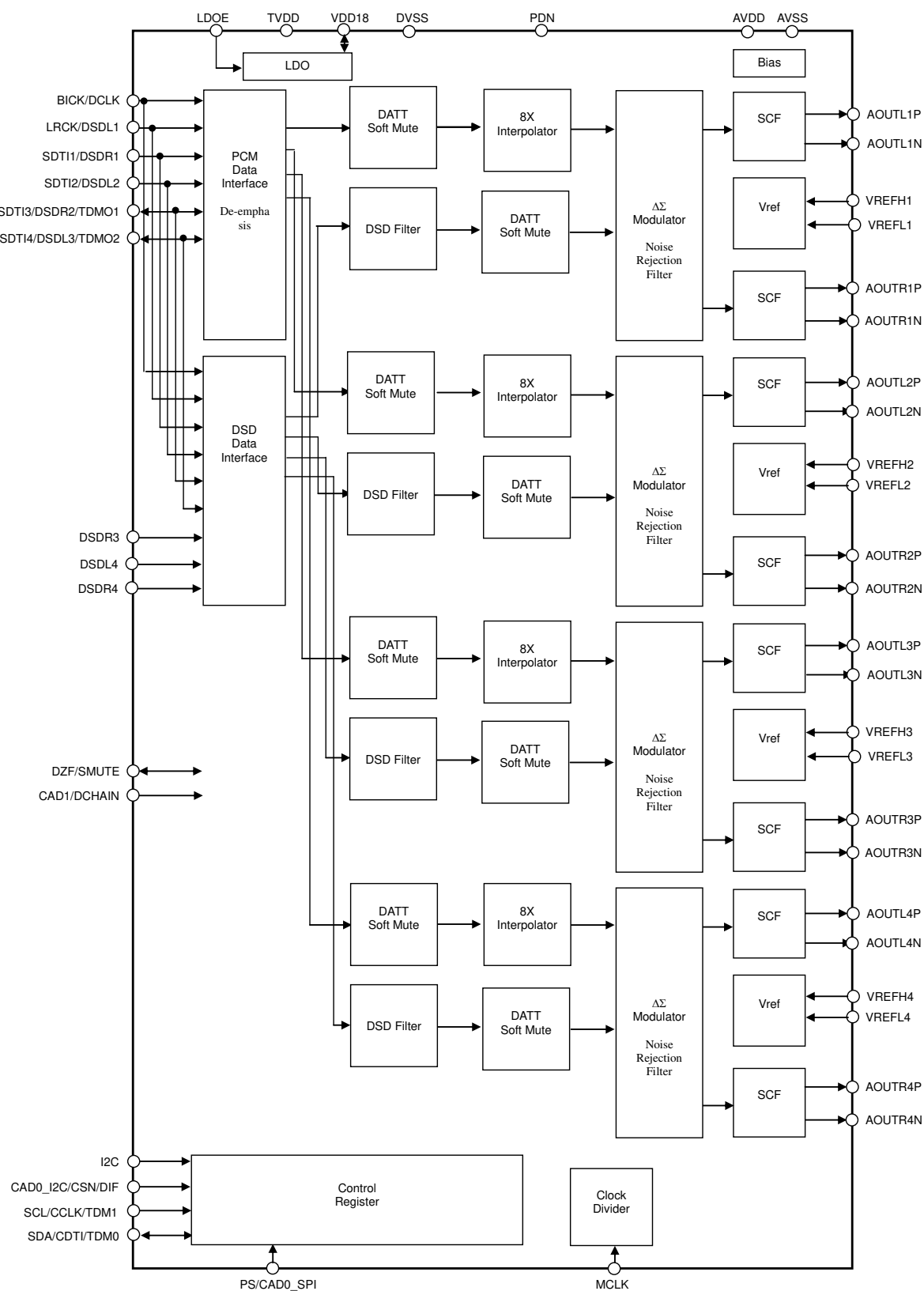
Figure 1. Block Diagram
