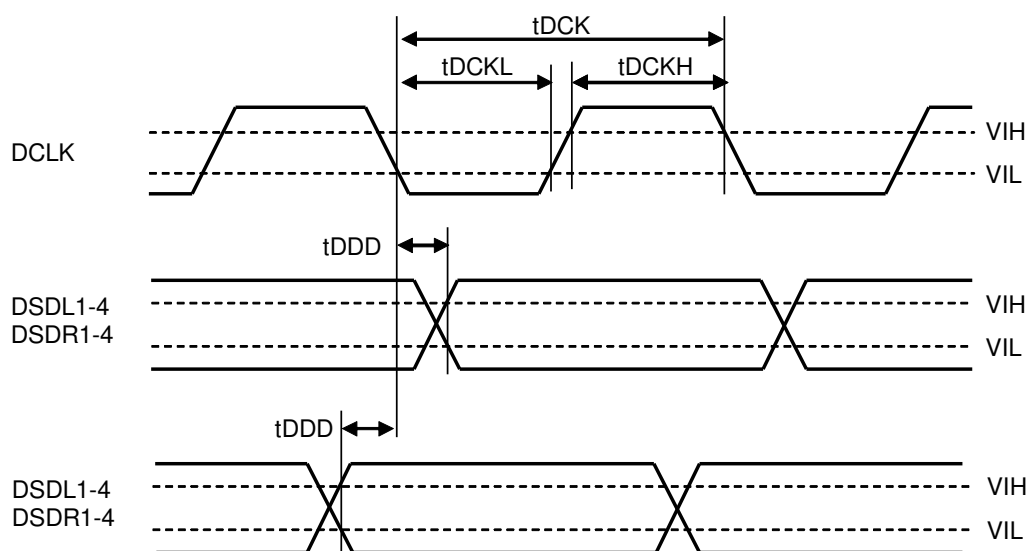
Figure 12. Audio Serial Interface Timing (DSD Normal Mode, DCKB bit = "0")
