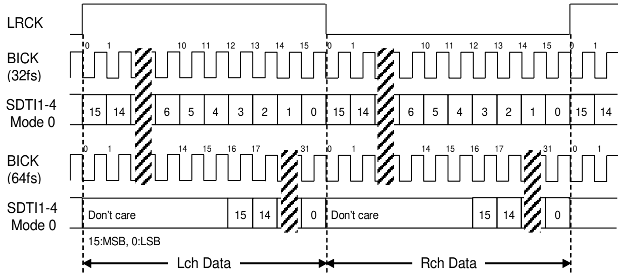
Figure 18. Mode 0 Timing
