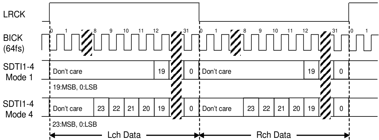
Figure 19. Mode 1/4 Timing
