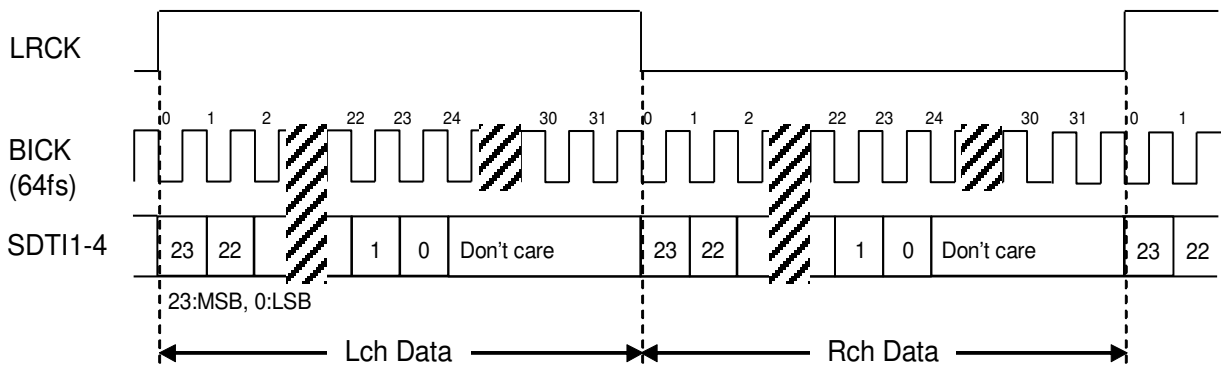
Figure 20. Mode 2 Timing
