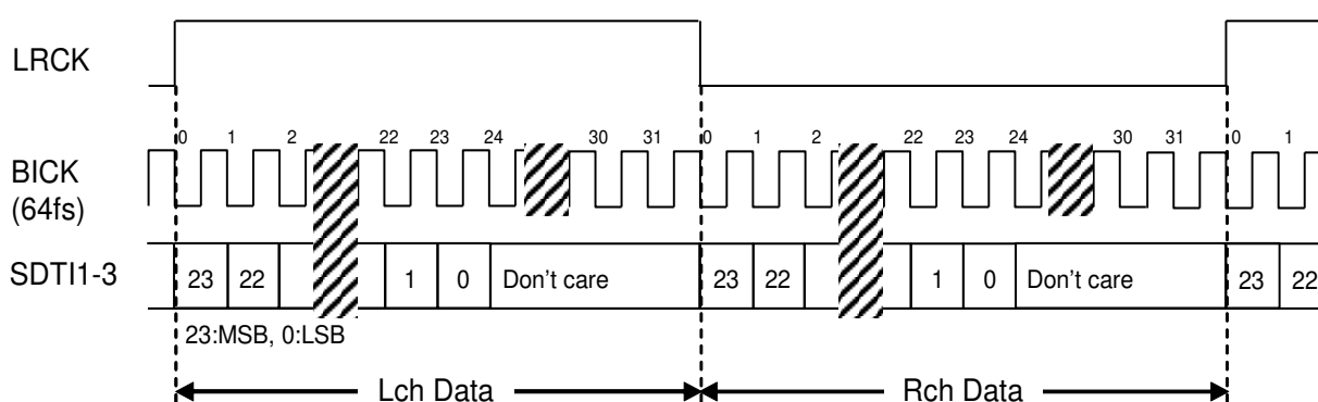
Figure 20. Mode 2 Timing
