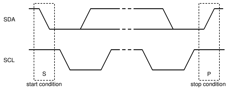
Figure 78. START and STOP Conditions
