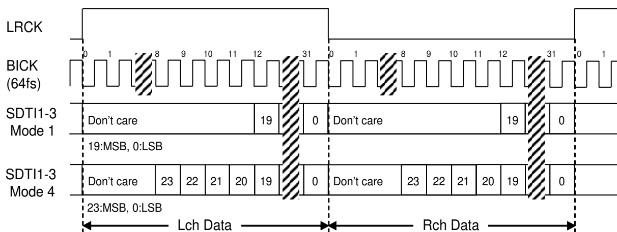
Figure 19. Mode 1/4 Timing
