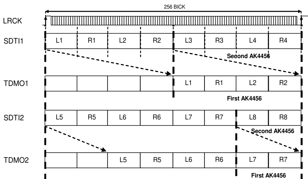
Figure 42. Daisy Chain (TDM256 Mode)
