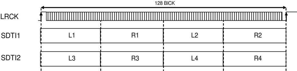
Figure 34. Data Slot in TDM128 Mode
