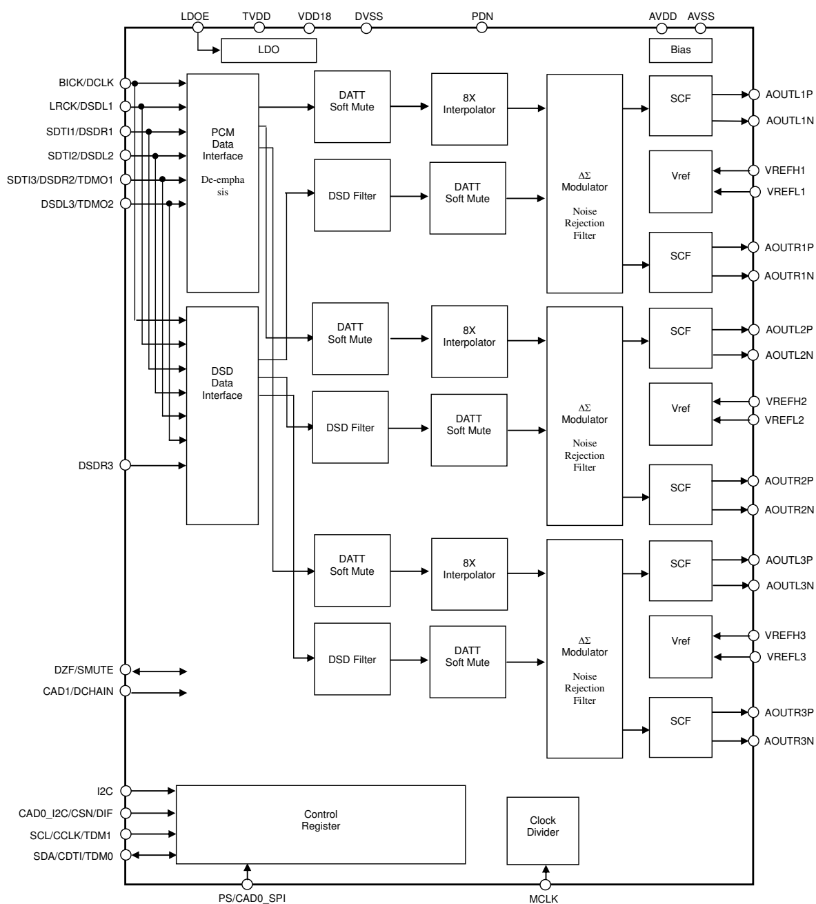
Figure 1. Block Diagram
