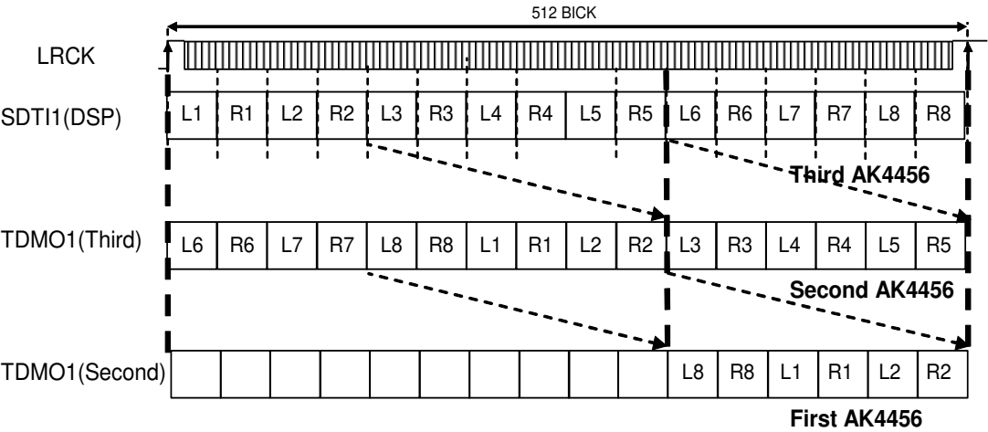
Figure 40. Daisy Chain for Three Devices (TDM512 Mode)
