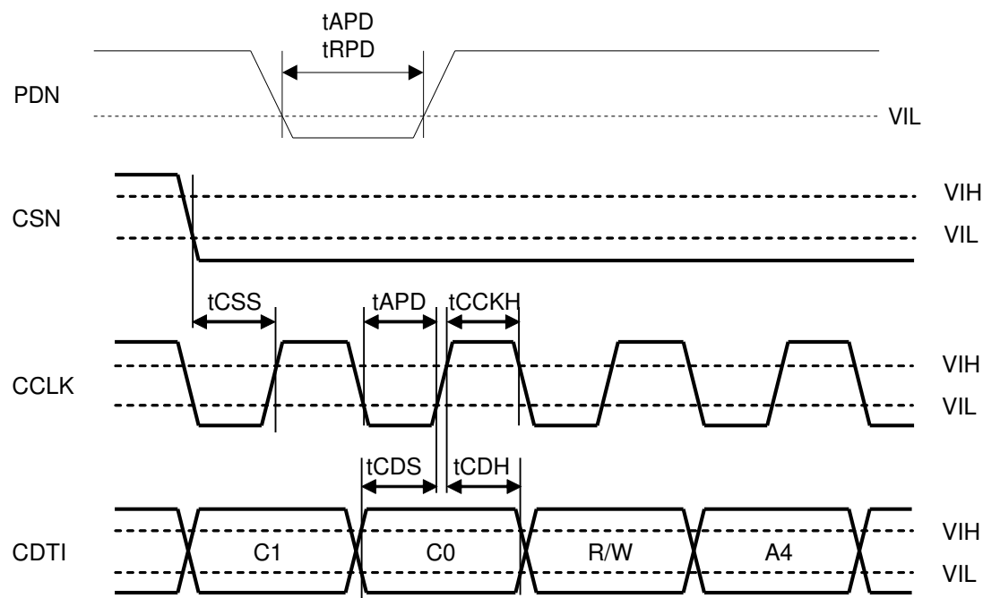
Figure 17. Power-down & Reset Timing
