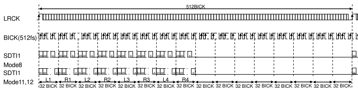
Figure 30. Mode 20/23/24 Timing
