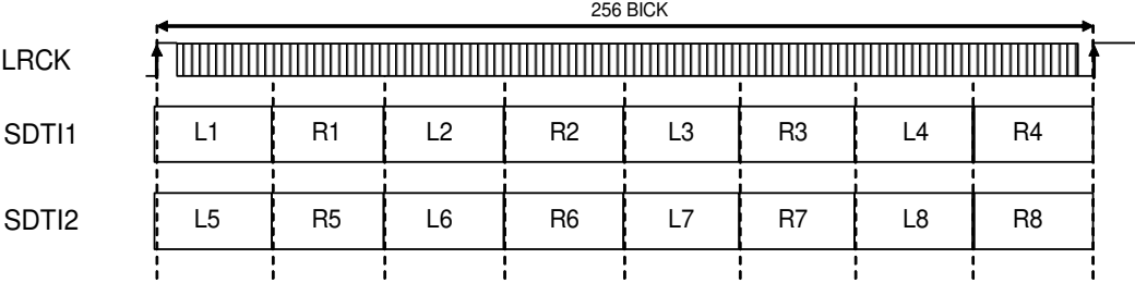
Figure 35. Data Slot in TDM256 Mode
