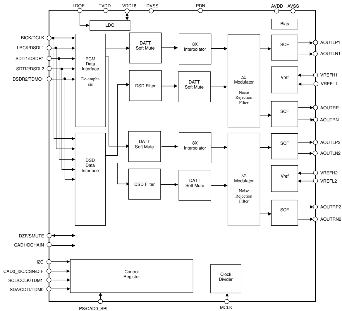
Figure 1. Block Diagram
