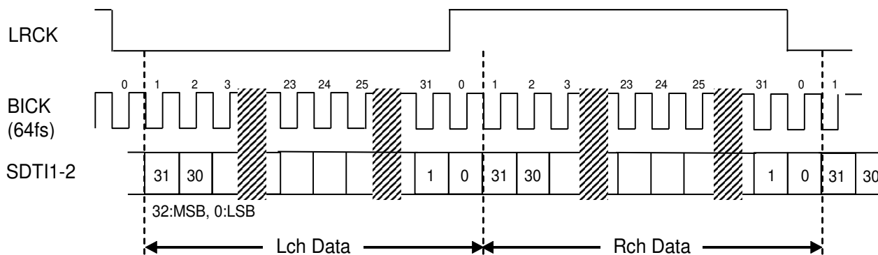
Figure 22. Mode 5/6 Timing
