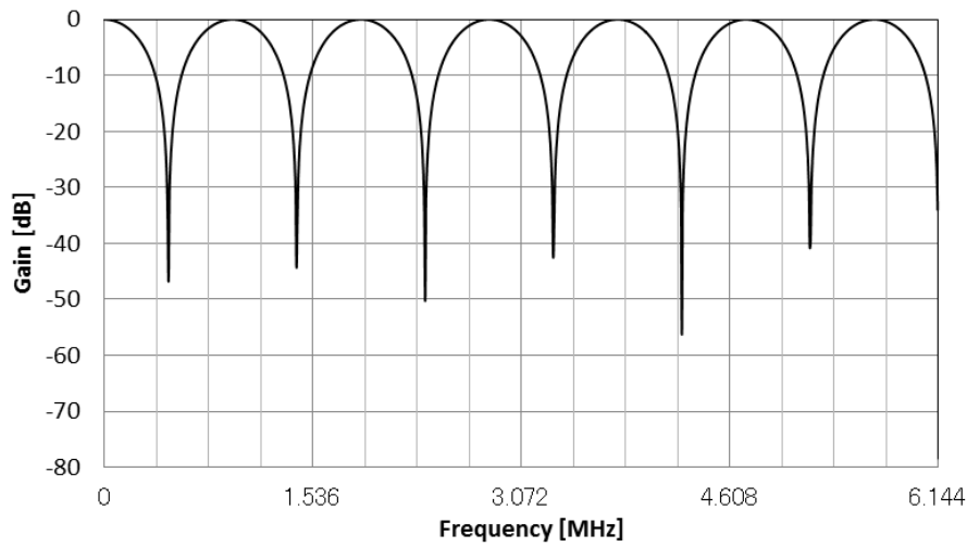
Figure 53. Model1 FIR Filter (DSD direct mode)
