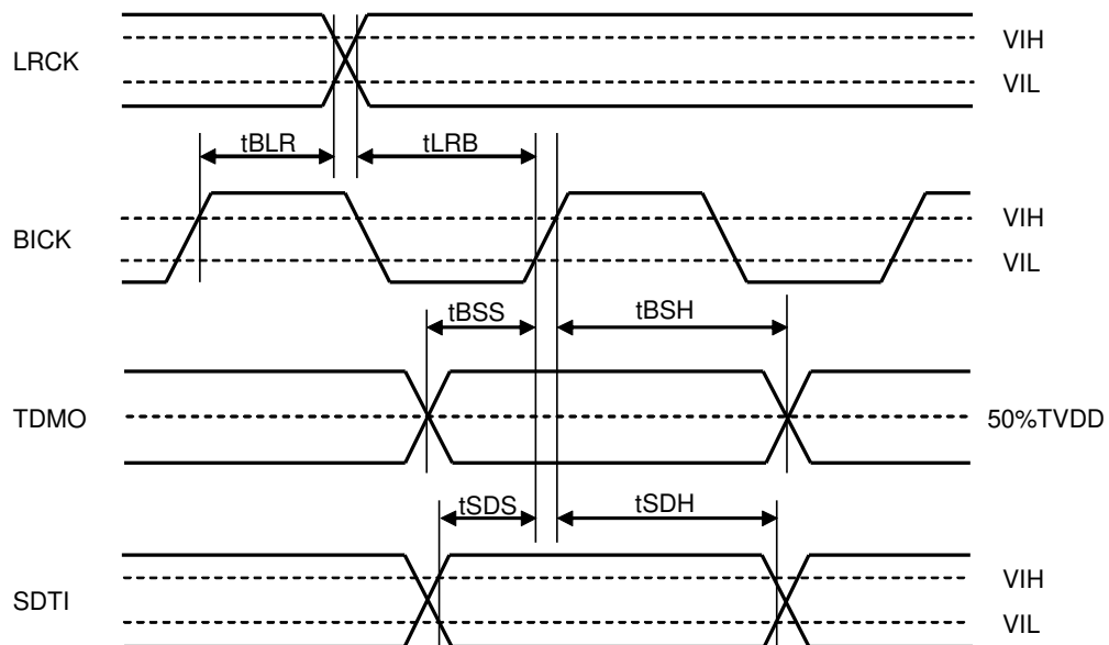
Figure 11. Audio Interface Timing (PCM Mode)
