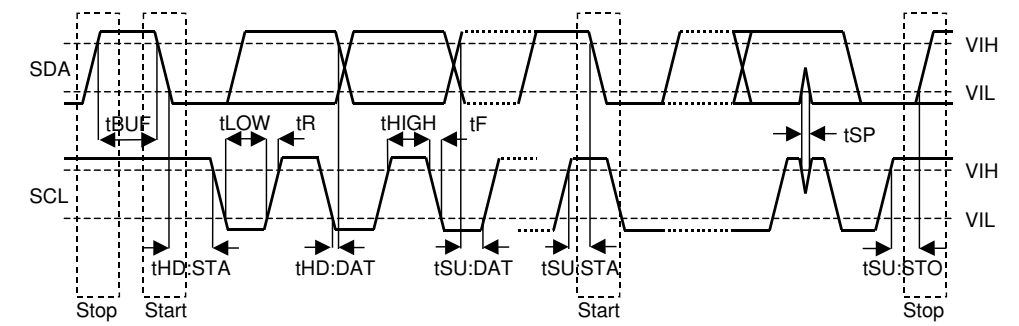
Figure 16. I²C Bus mode Timing
