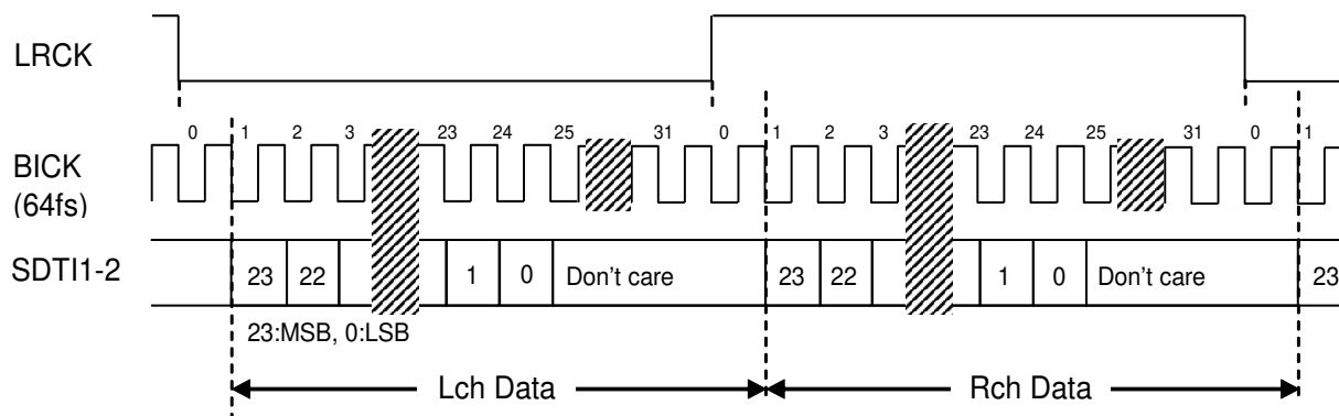
Figure 21. Mode 3 Timing
