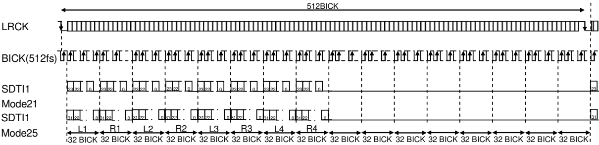
Figure 31. Mode 21/25 Timing
