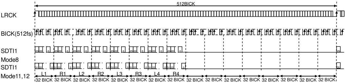
Figure 30. Mode 20/23/24 Timing
