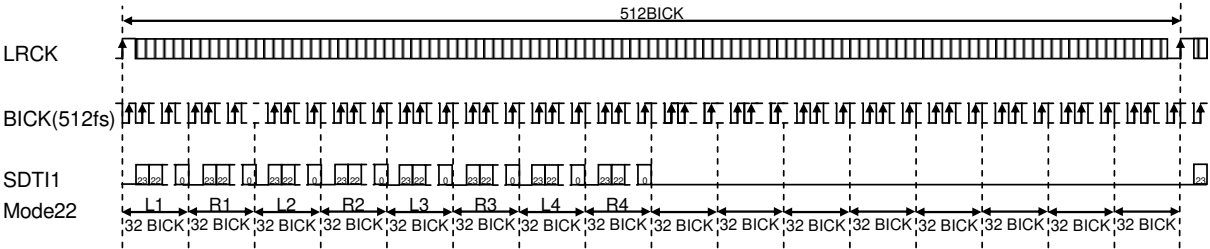
Figure 32. Mode 22 Timing
