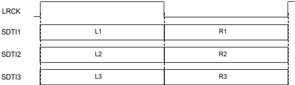
Figure 25. Data Slot in Normal mode
