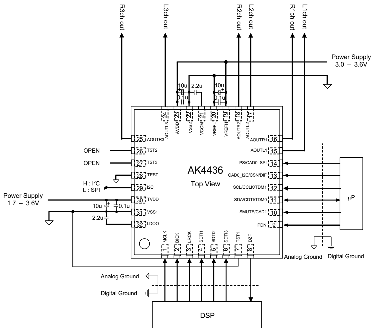
Figure 46. Typical Connection Diagram
