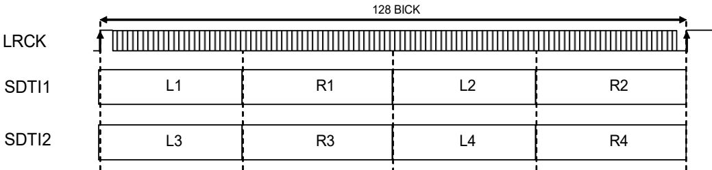
Figure 26. Data Slot in TDM128 mode
