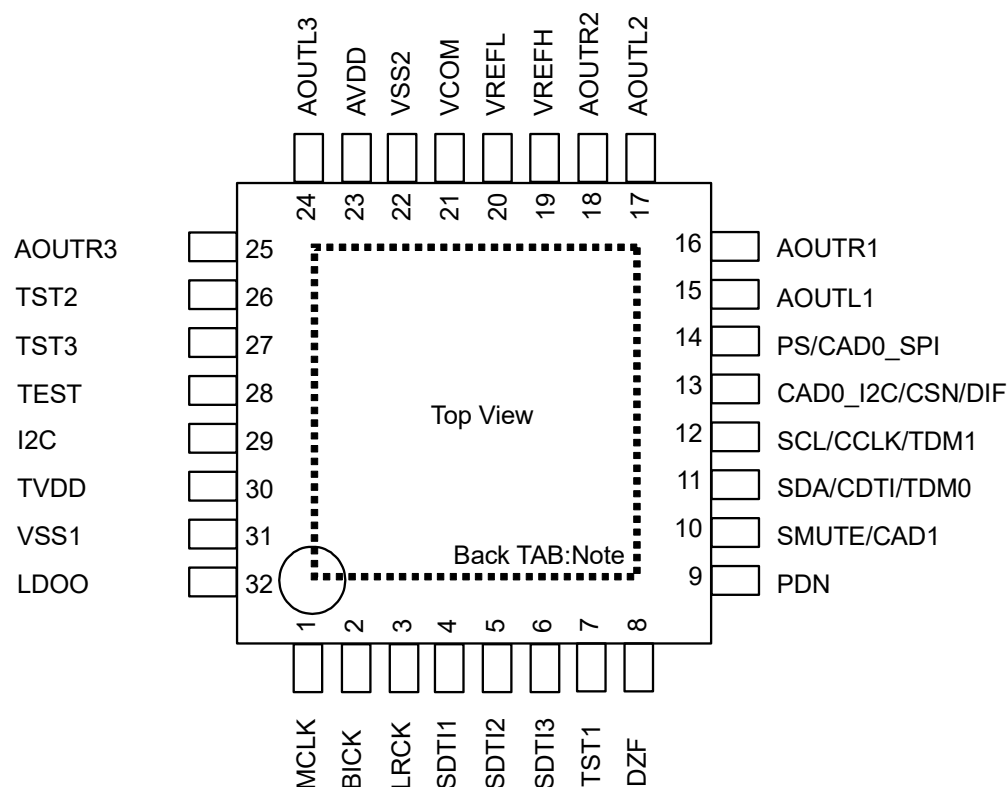
Figure 2. Pin Configuration
