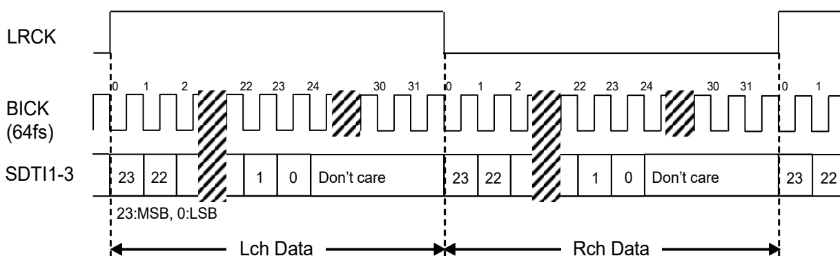
Figure 12. Mode 2 Timing
