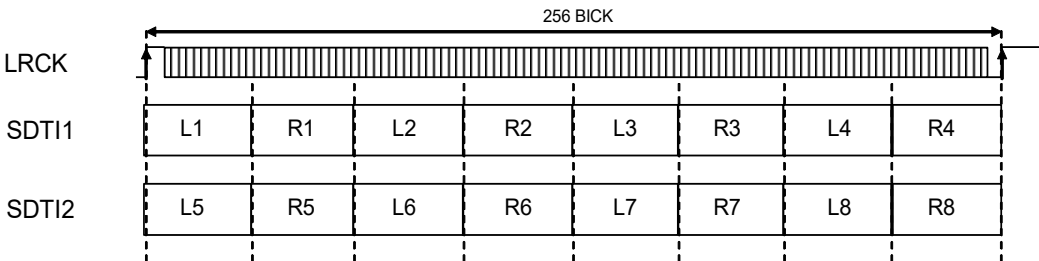
Figure 27. Data Slot in TDM256 mode
