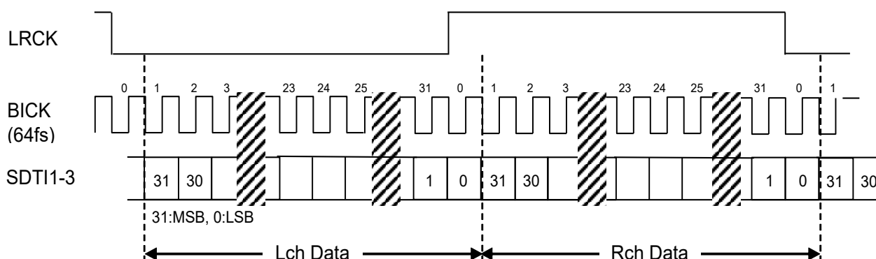
Figure 15. Mode 7 Timing
