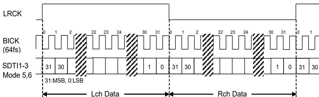
Figure 14. Mode 5/6 Timing
