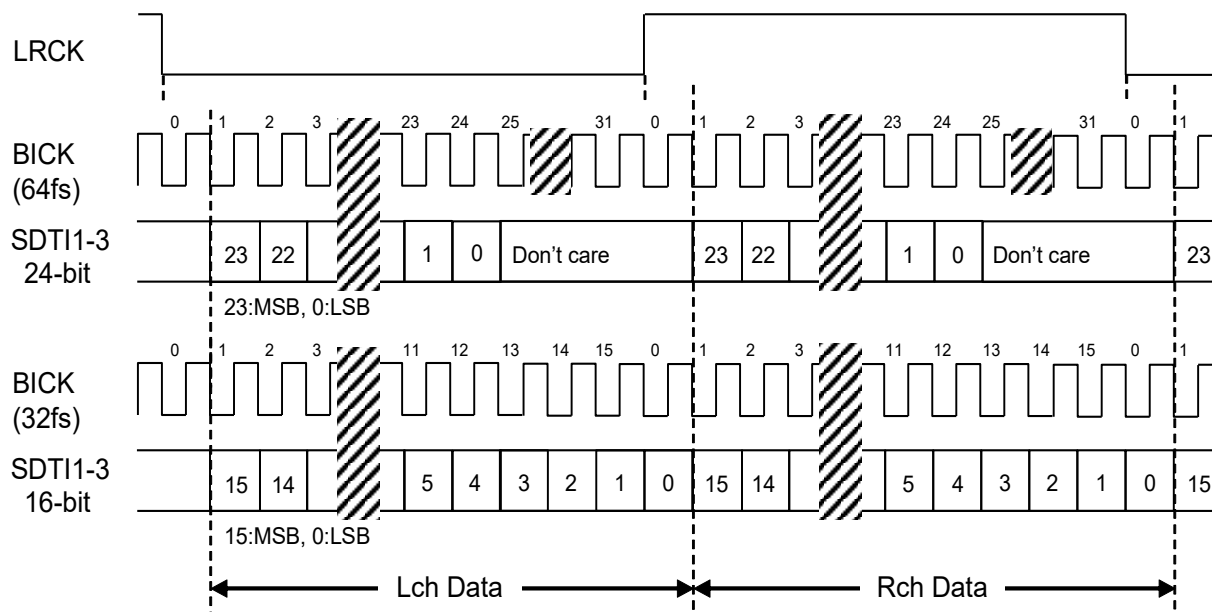
Figure 13. Mode 3 Timing
