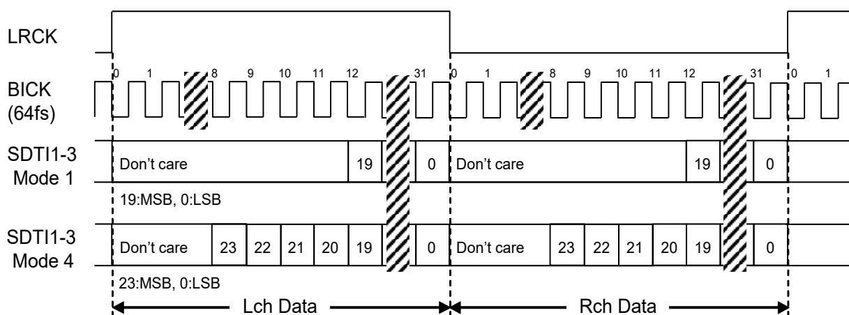
Figure 11. Mode 1/4 Timing
