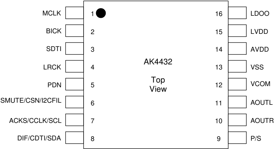
Figure 2. Pin Layout
