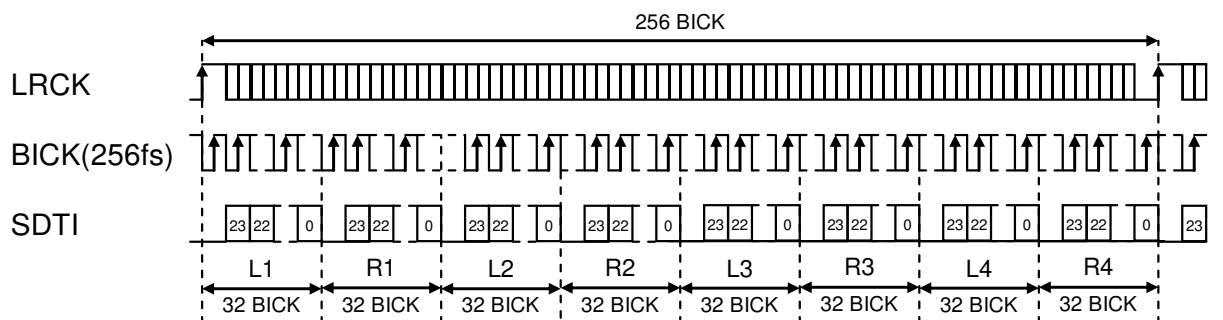
Figure 22. Mode 16 Timing
