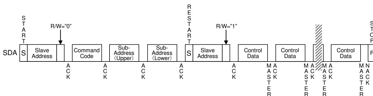
Figure 42. Data read sequence in I²C bus mode
