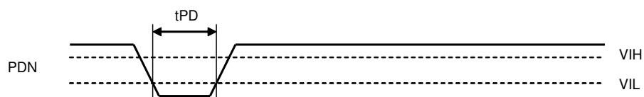
Figure 10. Power-down &amp; Reset Timing
