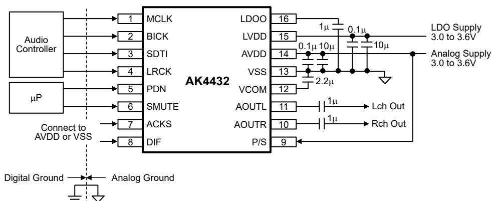
Figure 47. System Connection Diagram (Parallel mode)
