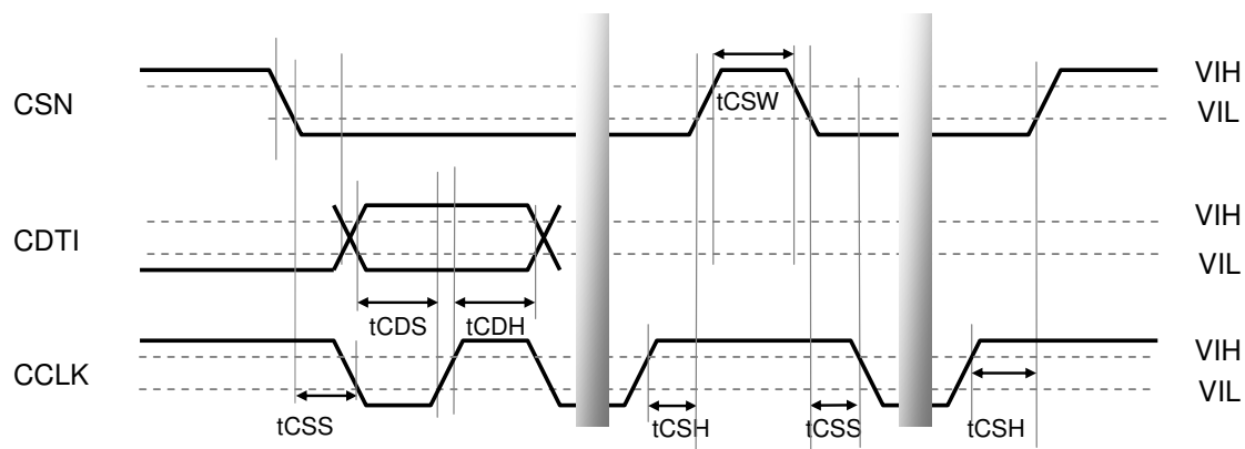
Figure 8. WRITE Data Input Timing (3-wire Serial mode)
