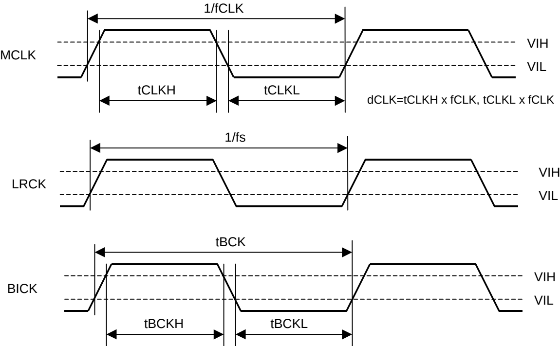
Figure 1. Clock Timing
