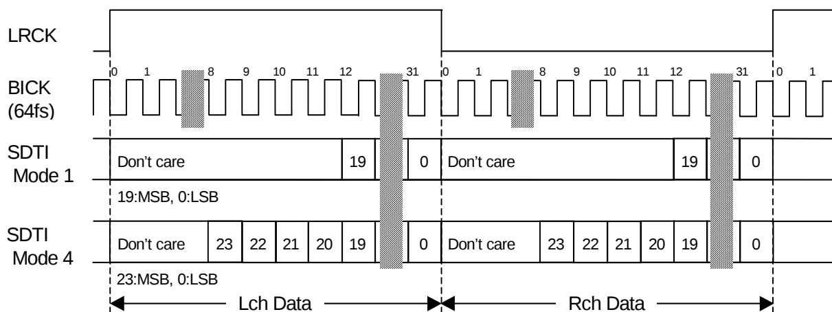
Figure 5. Mode 1/4 Timing
