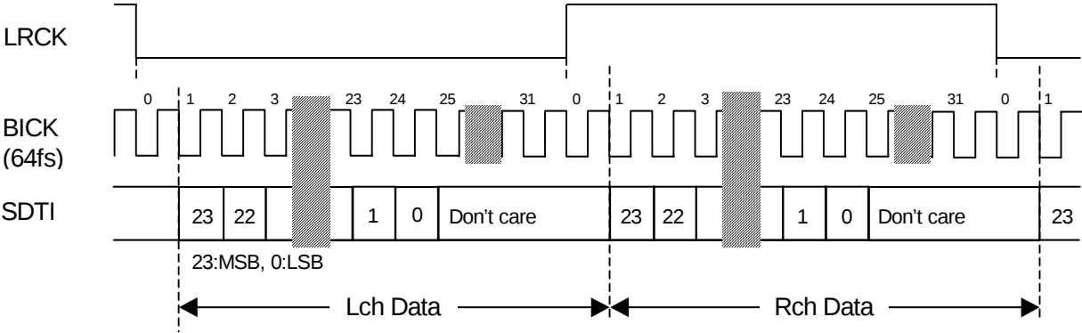
Figure 7. Mode 3 Timing
