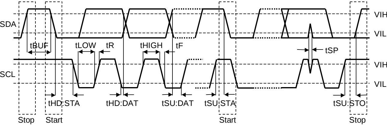
Figure 3. I²C Bus mode Timing
