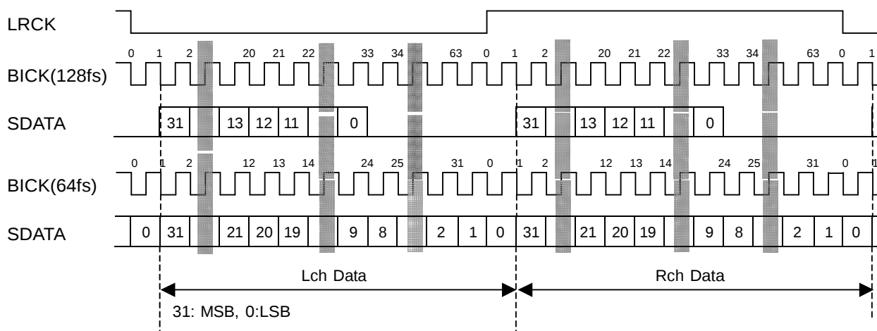
Figure 7. Mode 7 Timing
