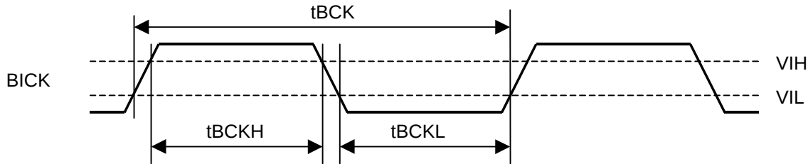
Clock Timing
