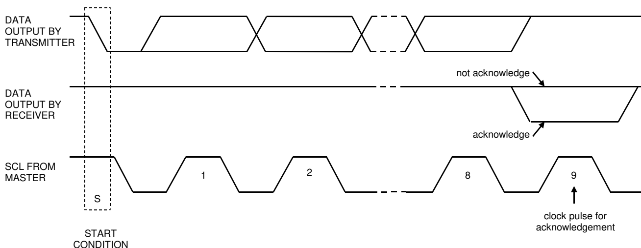
Figure 31. Acknowledge (I²C-bus)
