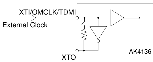
Figure 27. External Clock (OMCLK) Mode
