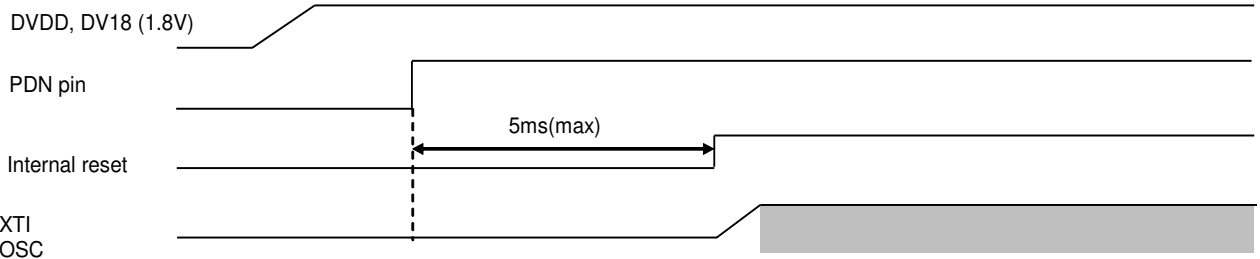
Figure 15. Power-up Sequence (Regulator Off Mode)
