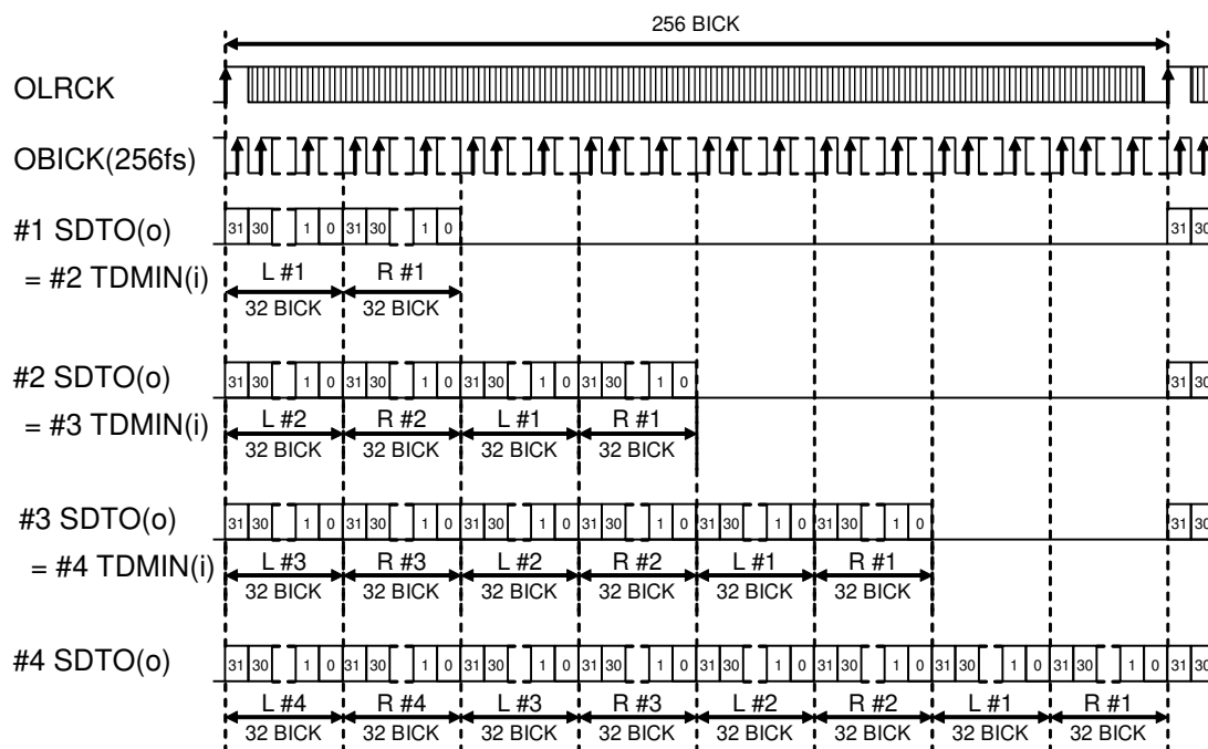
Figure 36. TDM Cascade
