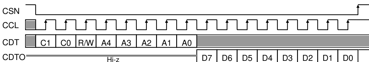
Figure 45. Read Operation
