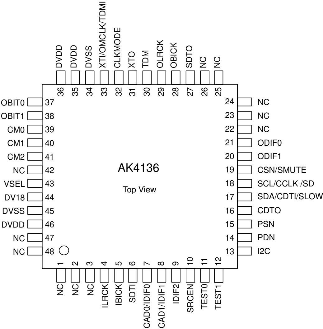
Figure 2. Pin Layout
