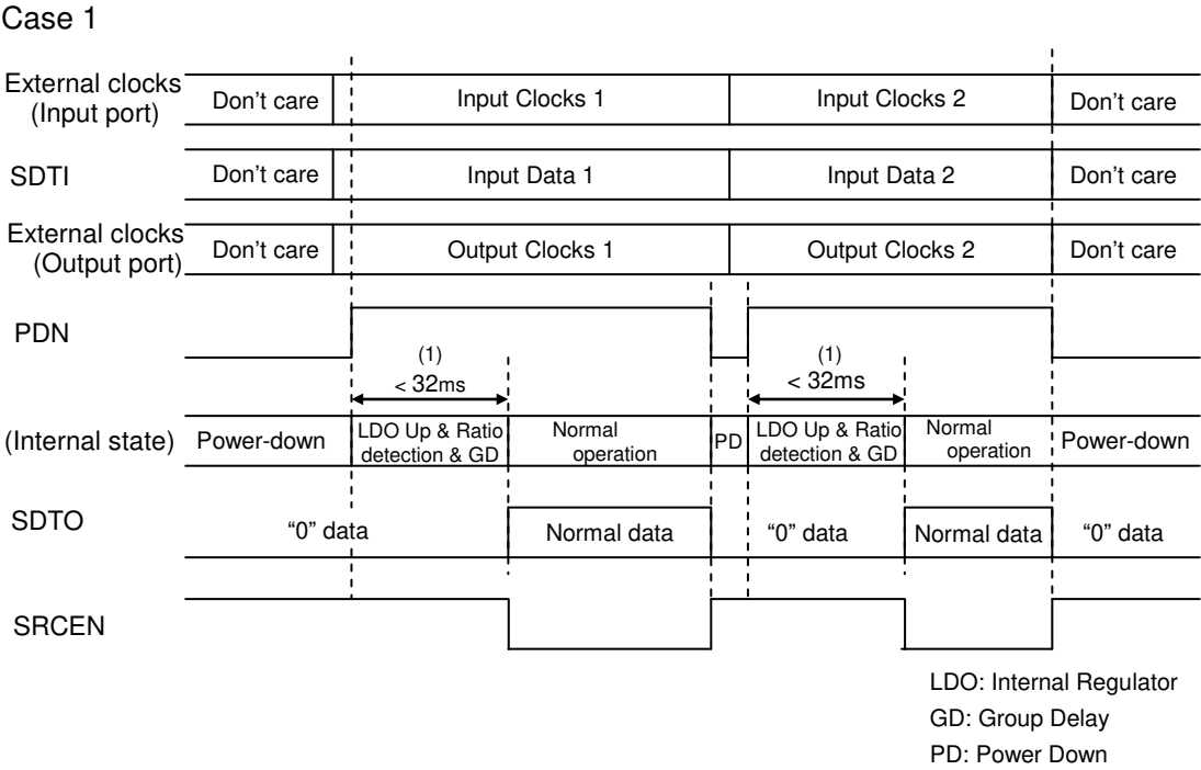
Figure 39. System Reset 1
