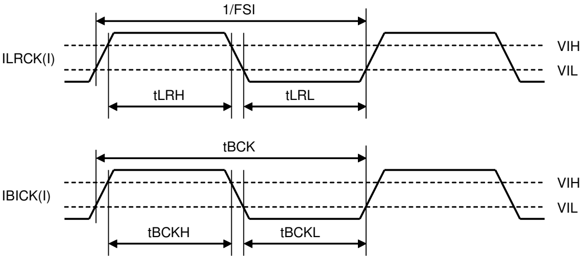
Figure 4. ILRCK, IBICK Clock Timing
