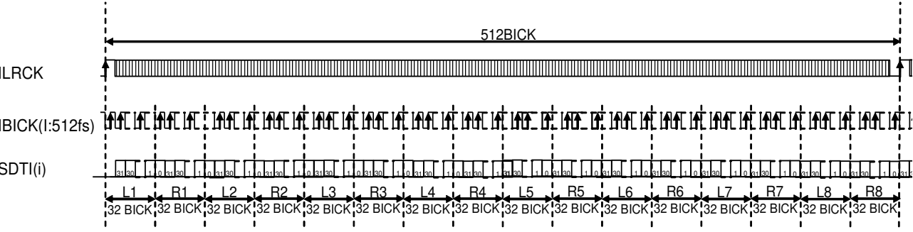
Figure 25. Mode7 Timing (32-bit I²S TDM512fs)
