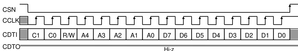
Figure 44. Write Operation
