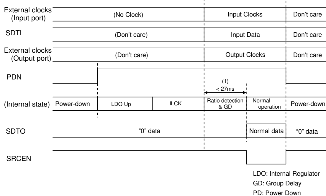
Figure 40. System Reset 2
