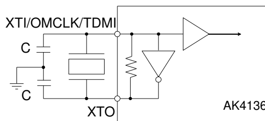
Figure 26. X'tal (XTI) Mode
