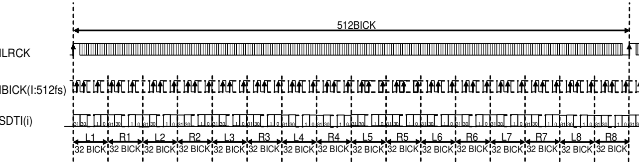
Figure 24. Mode6 Timing (32-bit MSB TDM512fs)
