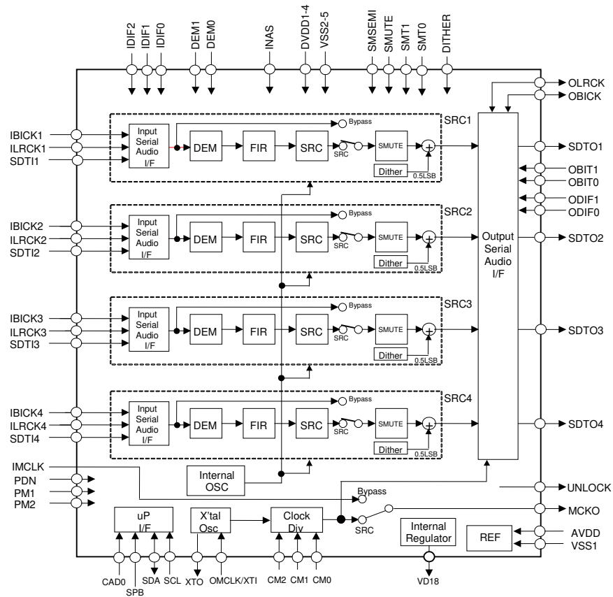
Figure 2. AK4128A Block Diagram (Asynchronous mode INAS pin = "H")
