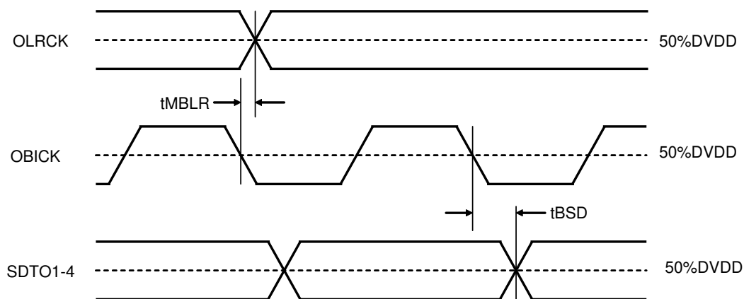
Figure 11. Output PORT Audio Interface Timing (TDM256 Master mode &amp; Stereo Master mode)
