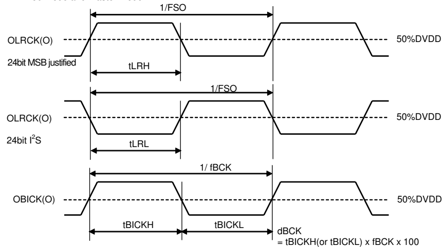
Figure 8. OLRCK, OBICK, Clock Timing (Master Mode)
