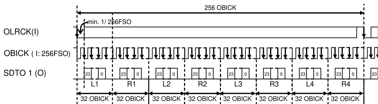
Figure 31. TDM 256 mode 24bit I²S Compatible Timing at Slave Mode (SDTO2-4: “L” outputs)
