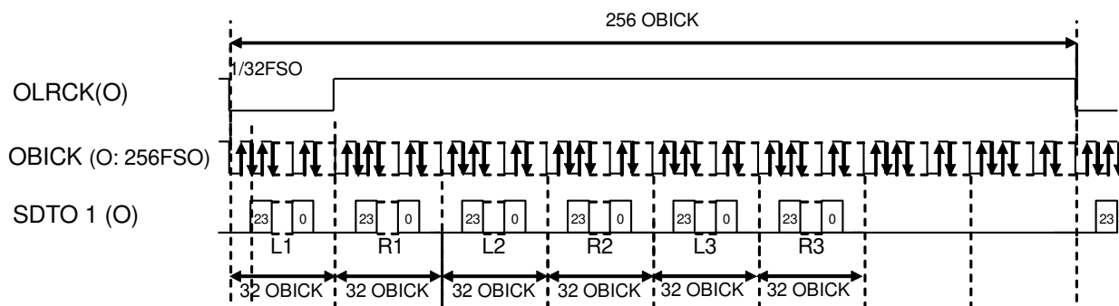
Figure 30. TDM 256 mode 24bit I²S Compatible Timing at Master Mode (SDTO2-4: “L” outputs)
