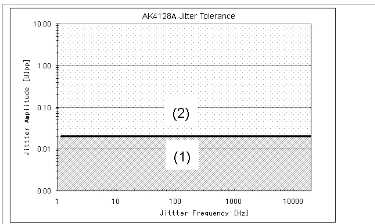
Figure 50. Jitter Tolerance
