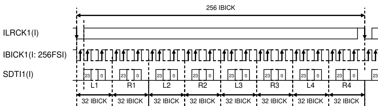
Figure 20. Mode 6 Timing (TDM, I 2 S, SDTI2-4: Don't care)
