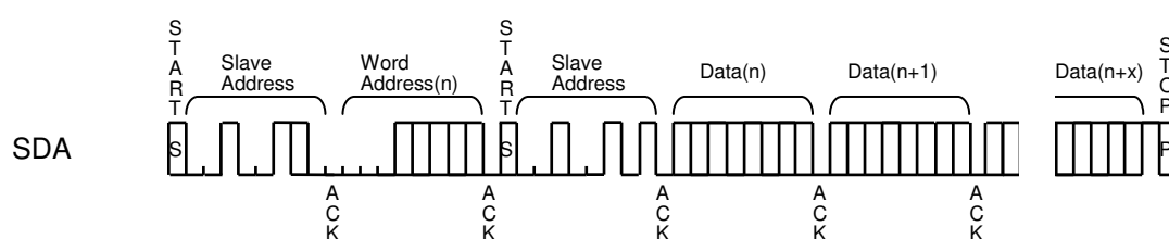
Figure 47. RANDOM READ
