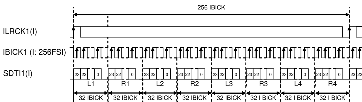
Figure 19. Mode 5 Timing (TDM, 24bit, MSB justified, SDTI2-4: Don't care)
