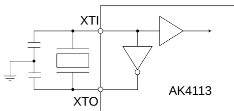
Figure 13. X'tal mode
