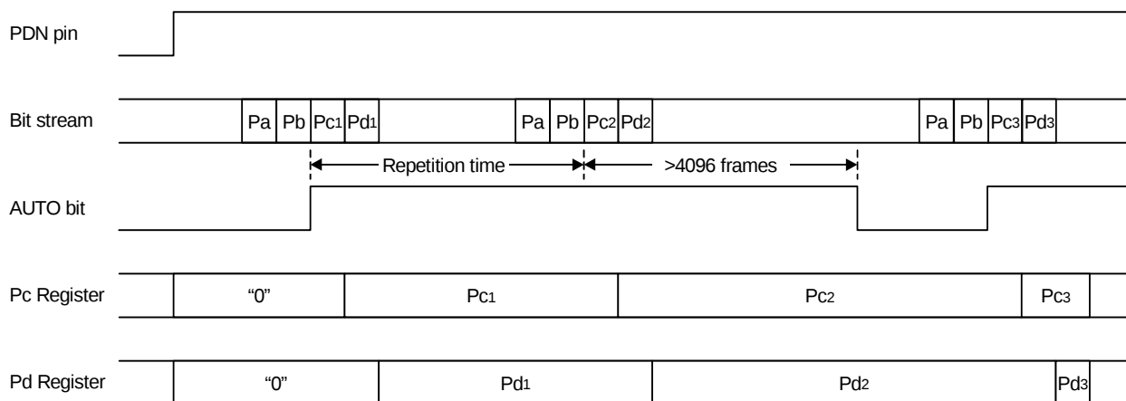
Figure 42. Timing Example 1
