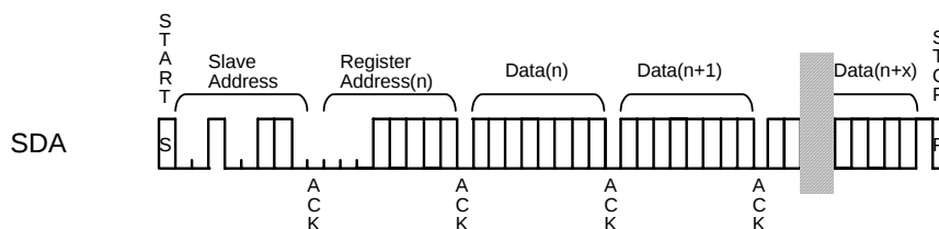
Figure 38. WRITE Operation
