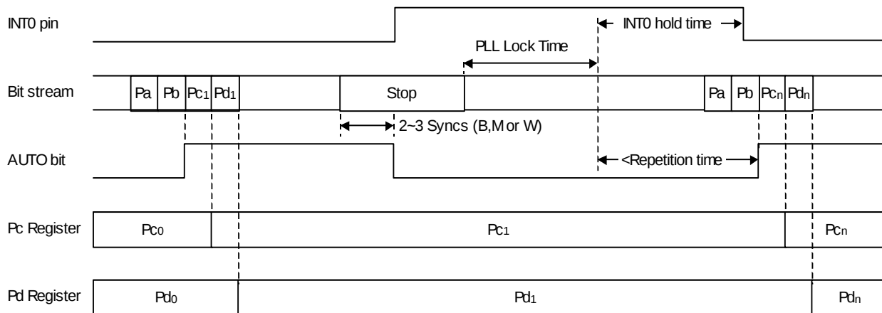
Figure 43. Timing Example 2
