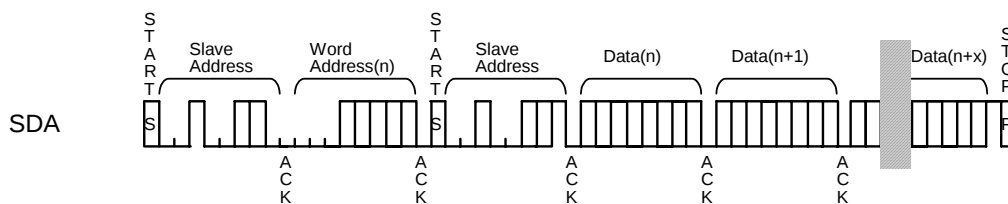
Figure 40. RANDOM READ
