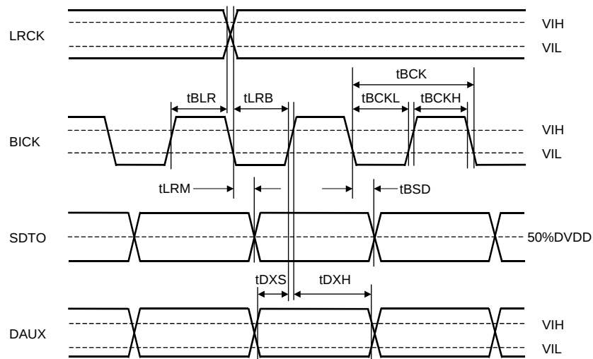
Figure 3. Clock Timing
