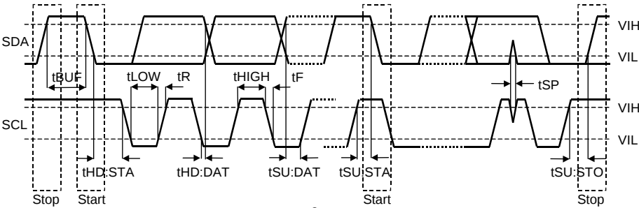
Figure 10. I²C Bus Mode Timing
