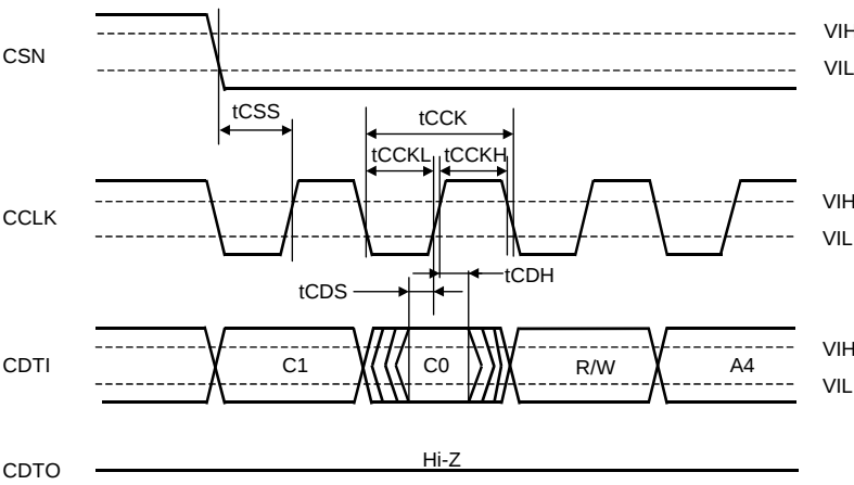
Figure 6. WRITE/READ Command Input Timing (4-wire serial mode)
