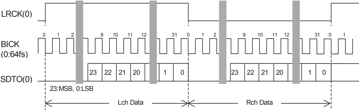
Figure 6. Mode 3 Timing
