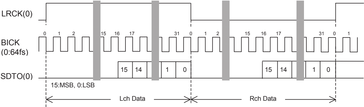
Figure 5. Mode 0 Timing
