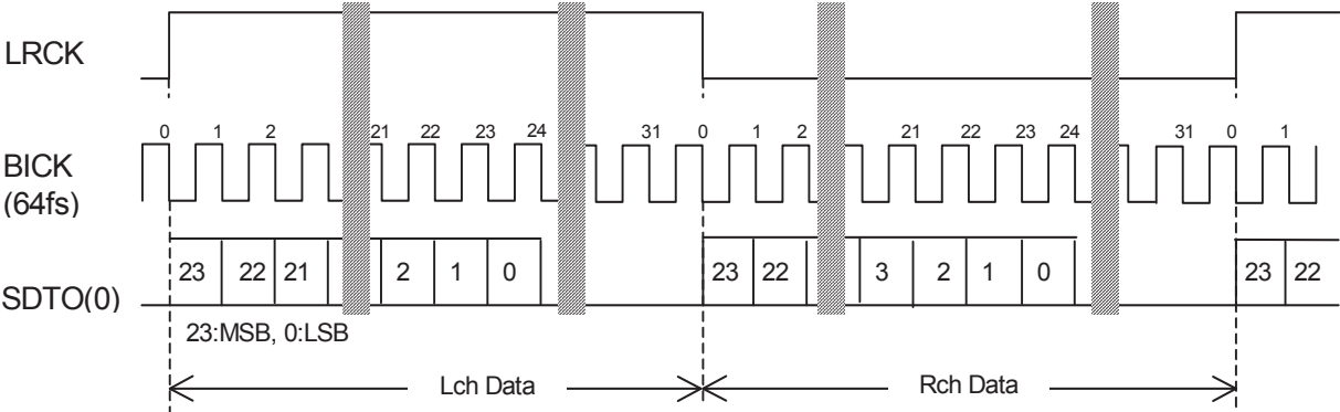
Figure 7. Mode 4, 6 Timing
