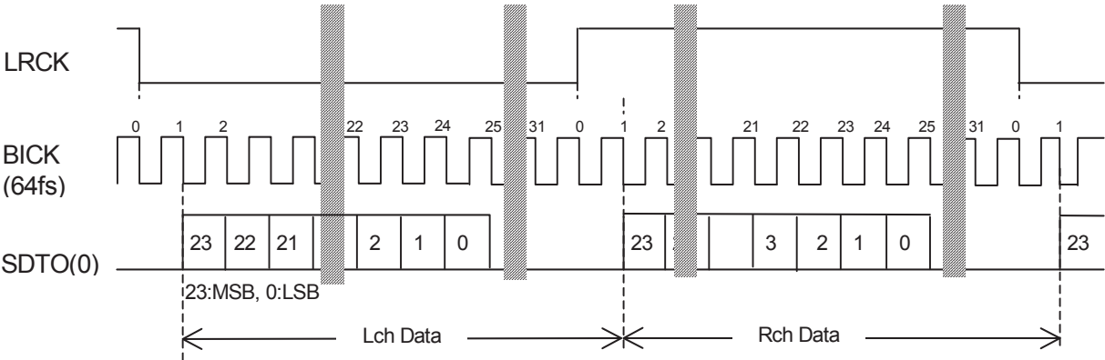
Figure 8. Mode 5, 7 Timing
