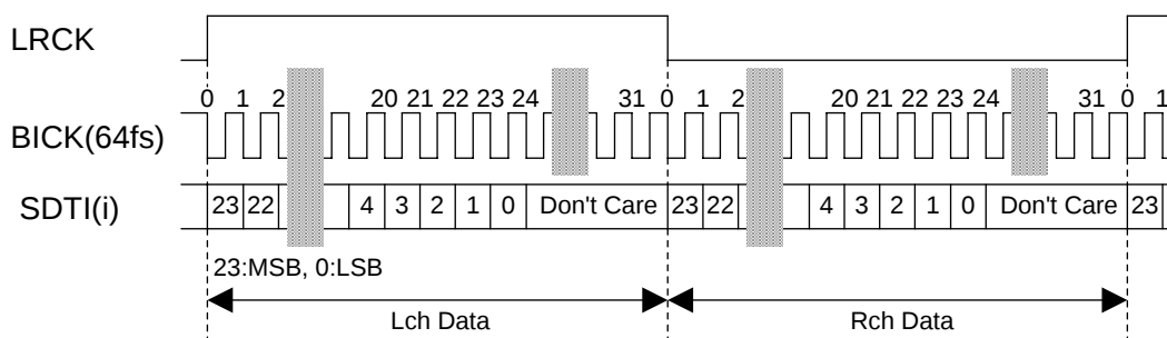
Figure 12. Mode 2 Timing
