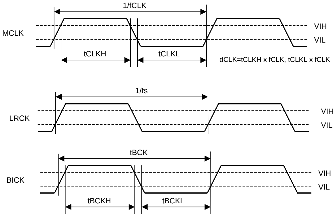
Figure 3. Clock Timing
