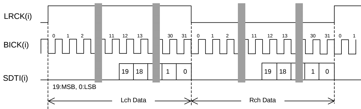
Figure 10. Mode 2 Timing
