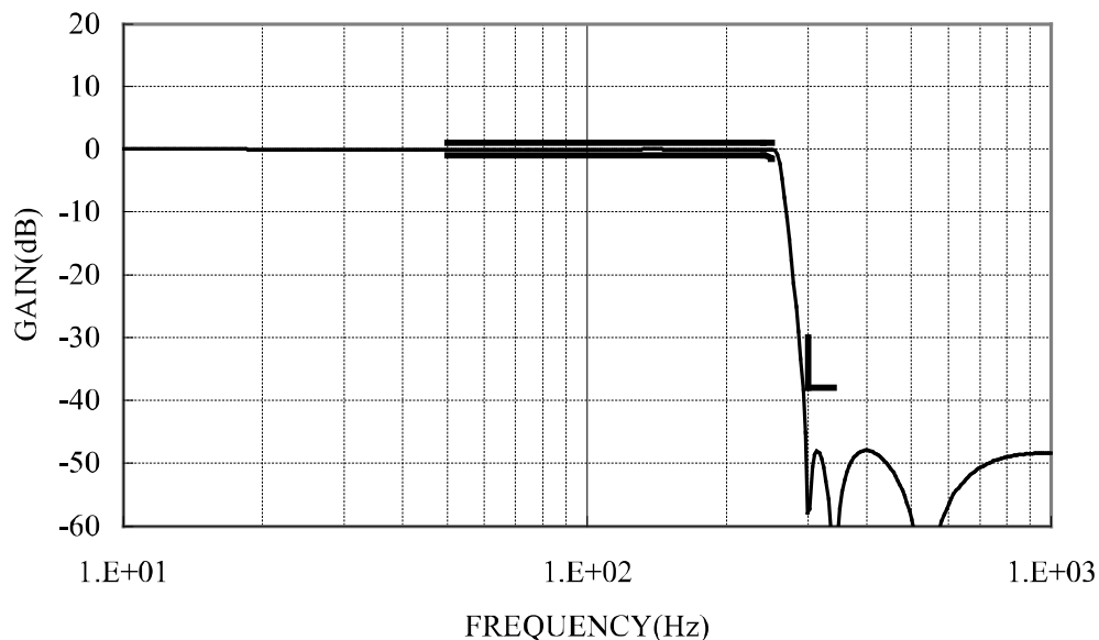
Fig.5 Sub-Audio response characteristics
