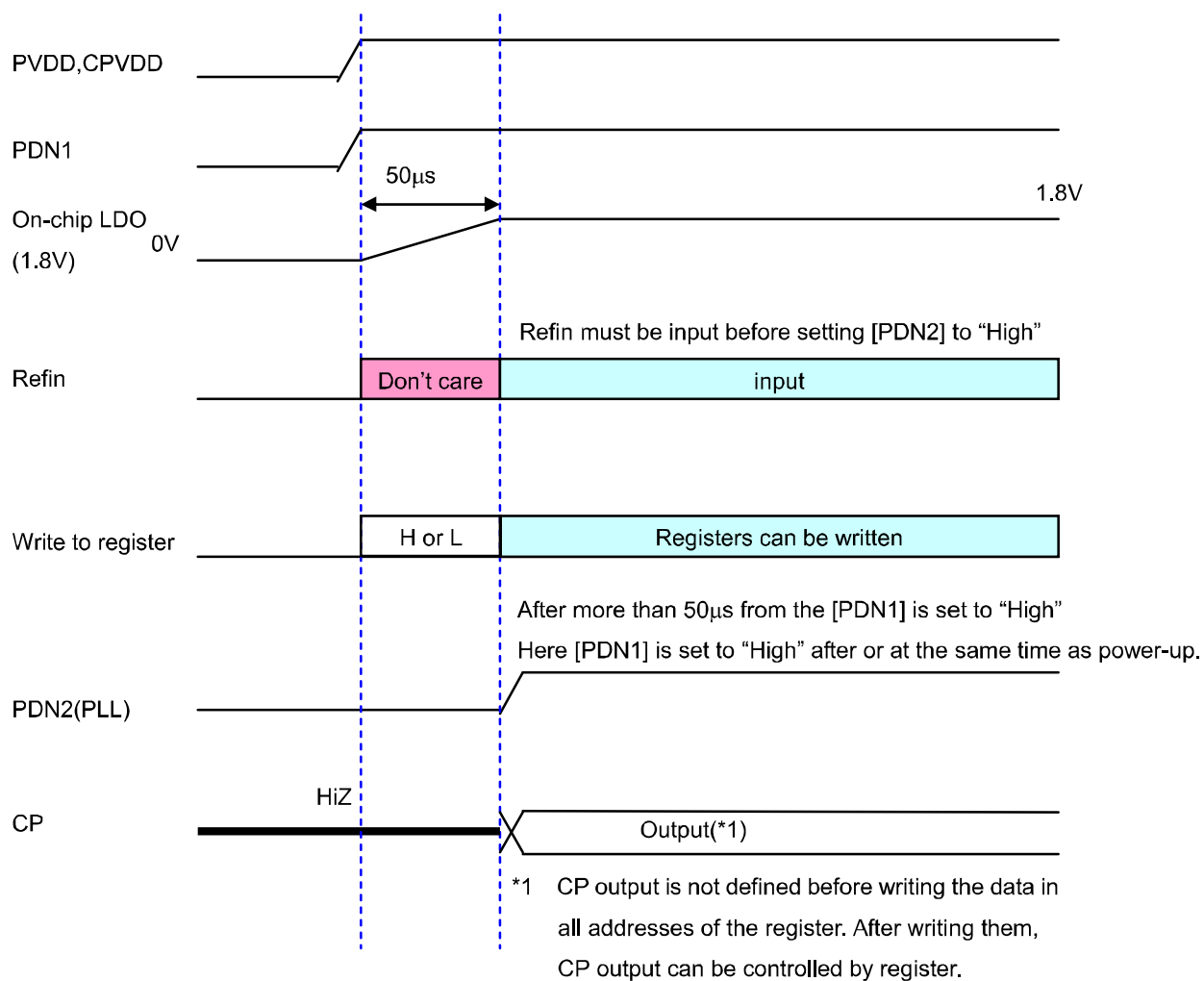
Fig. 13 Power Sequence
