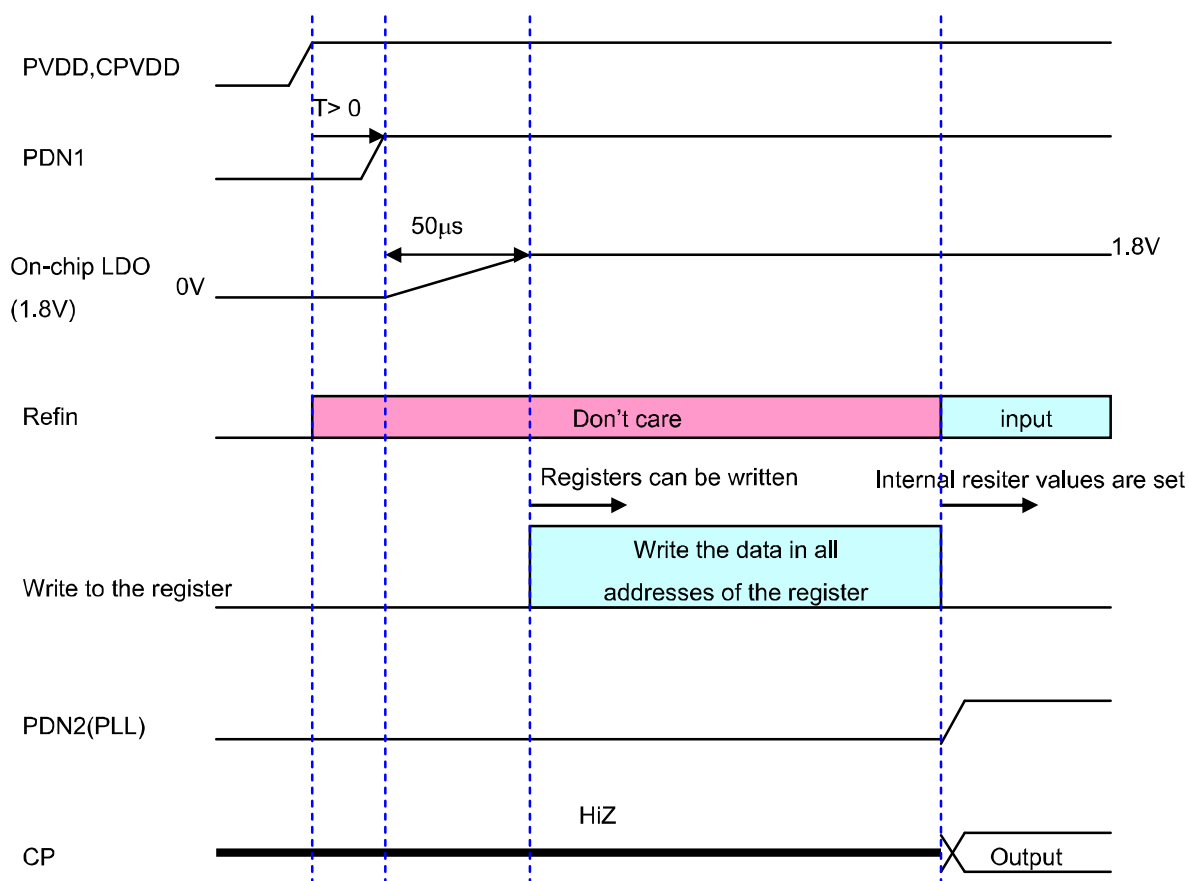
Fig. 12 Recommended Power Sequence
