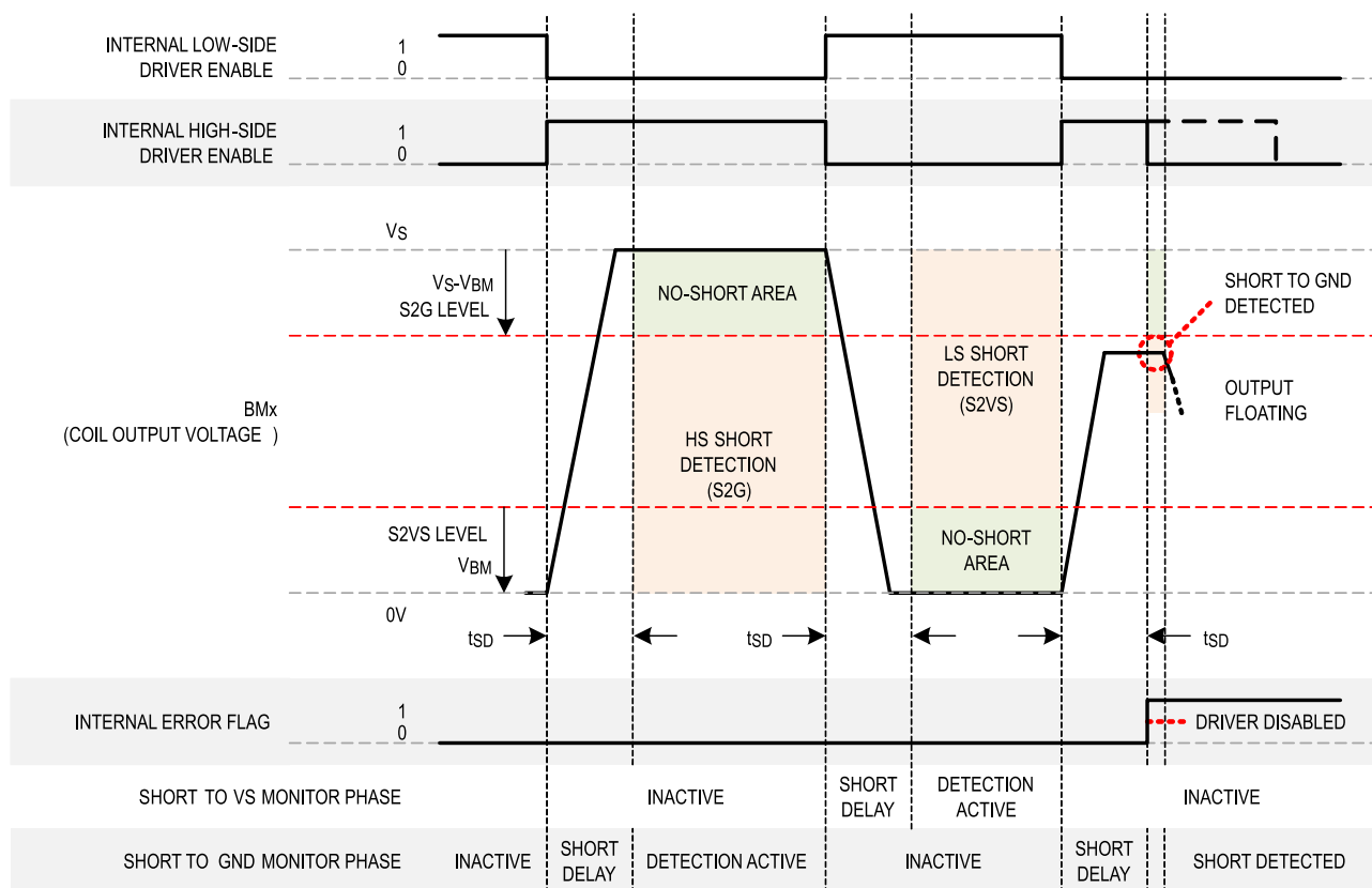
Figure 18: Short Detection (U/V/W Outputs)
