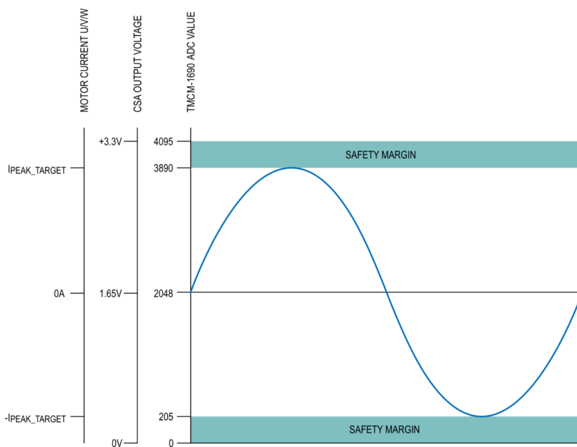
Figure 14: Direct Coil Current Sense Resistor Selection
