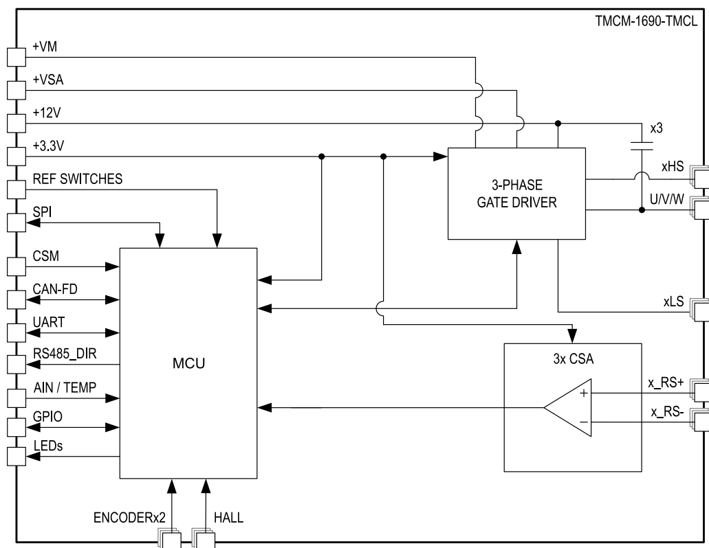
Figure 4: TMC1690-TMCL System Architecture
