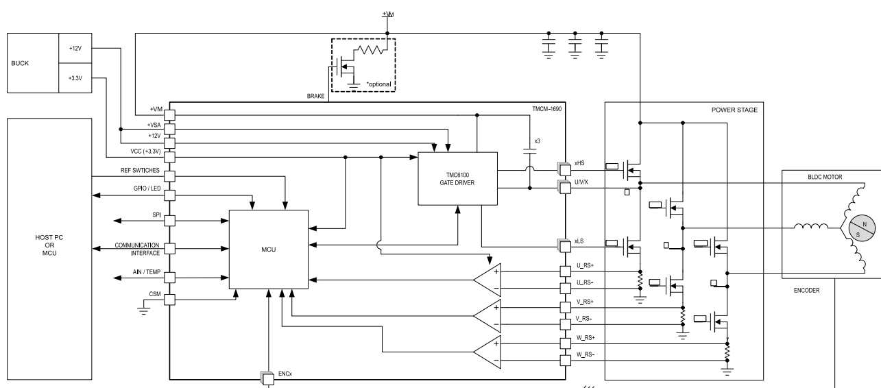
Figure 16: Bottom Shunt Current Sense
