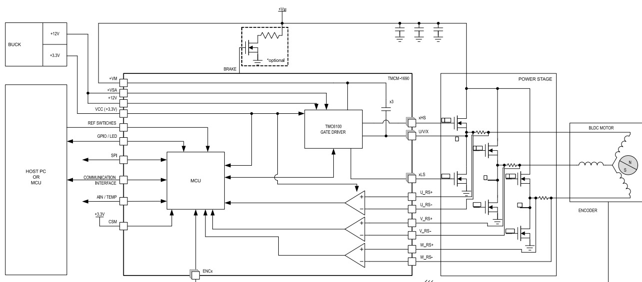
Figure 15: Inline Current Sense
