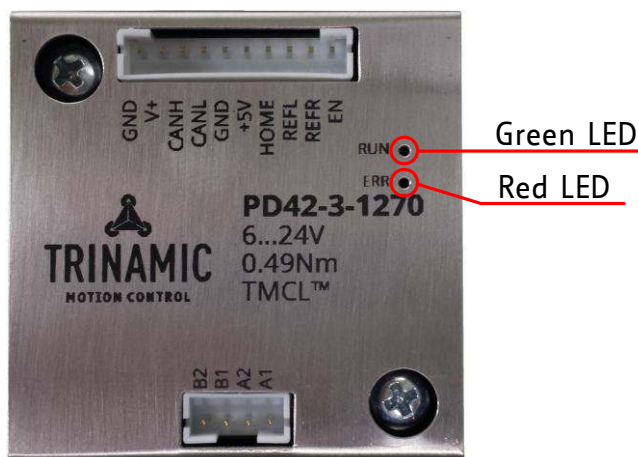
Figure 10: TCM-1270 LED colors and location
