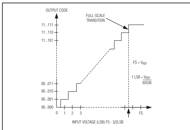
Figure 8. MAX1165/MAX1166 Transfer Function
