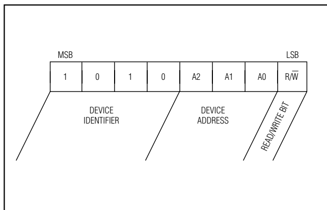
Figure 4. Slave Address
